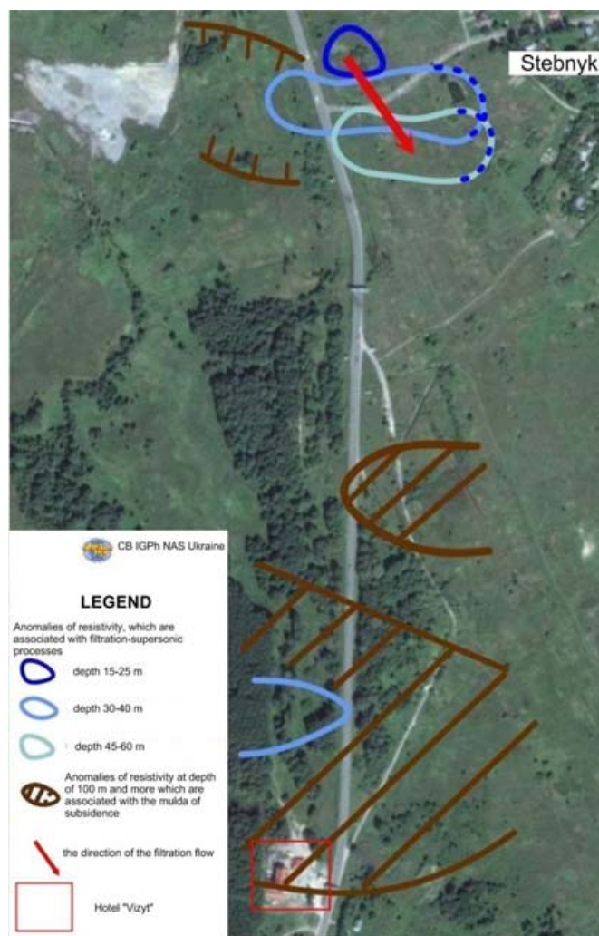
Fig. 8. Scheme of anomalous zones location for electromagnetic soundings along Skhidnytsia-Pisochne highway
