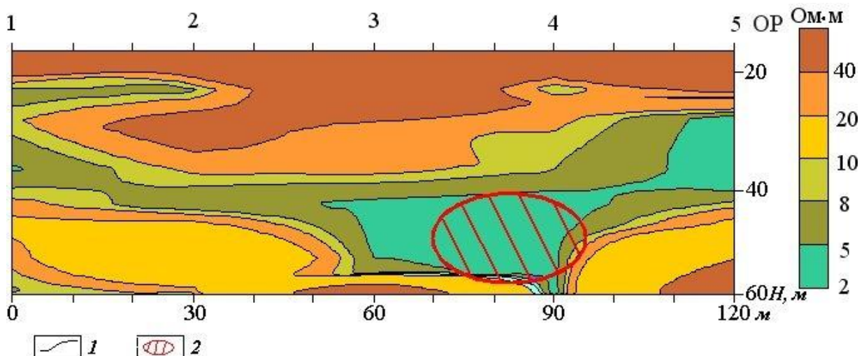
Fig. 5. Geoelectric cross-section for 2009 observations corresponds with 2017 observations on the profile I – I, OP d1–d4 1 – isooms; 2 – an anomalous zone
