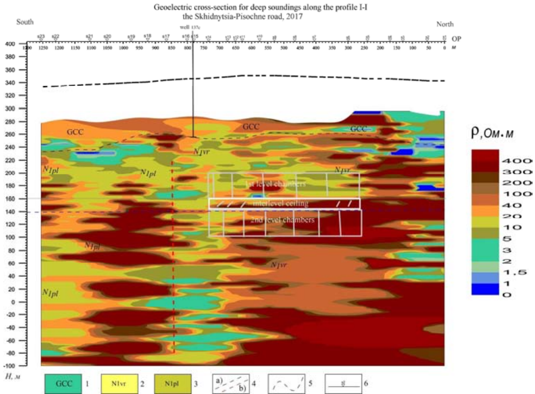
Fig. 6. Geoelectric cross-section for deep soundings along the profile I-I 1 – GCC sediments; 2 – Vorotyscha suite sediments; 3 – Polyanytsia suite sediments; 4 – lithological boundaries; 5 – Earth’s surface; 6 – OP
