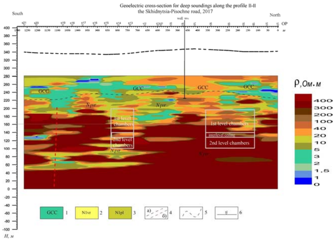
Fig. 7. Geoelectric cross-section of deep soundings along the profile II – II. 1 – GCC sediments; 2 – Vorotyscha suite sediments; 3 – Polyanytsia suite sediments; 4 – lithological boundaries; 5 – Earth’s surface; 6 – OP
