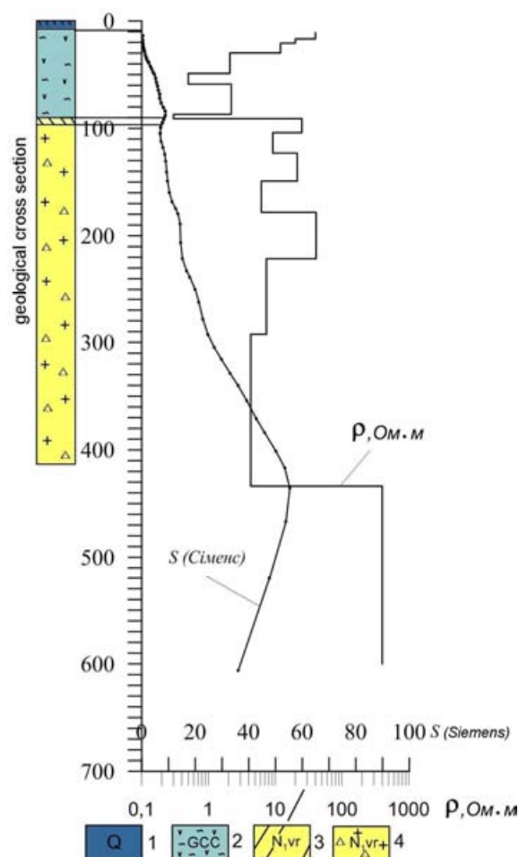
Fig. 2. Observation results by TDEM method on the parametric well No.137 1 – Quaternary sediments; 2 – sediments of gypsum-clay cap (GCC): clay, gypsum, sandstones, sandy loam, breccias; 3 – conductive zone of above-salt waters; 4 – Vorotyscha suite sediments: potassium and halite salts, clay, siltstones, sandstones
