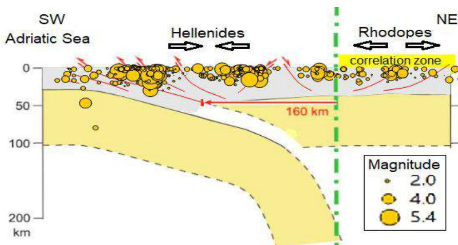
Fig. 11. Cross section of tectonic structures of Dinarides-Hellenides with earthquake hypocenters (modified from [Handy, et al., 2019; Nagel, et al., 2011])
