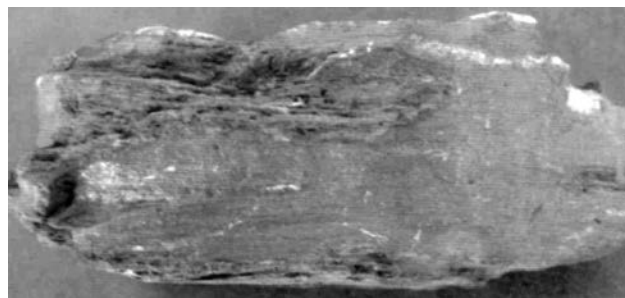
Fig. 6. Oxidized ferruginous quartzite with the ore gold-bearing veinlets [Квасниця, Латиш, 1996]
