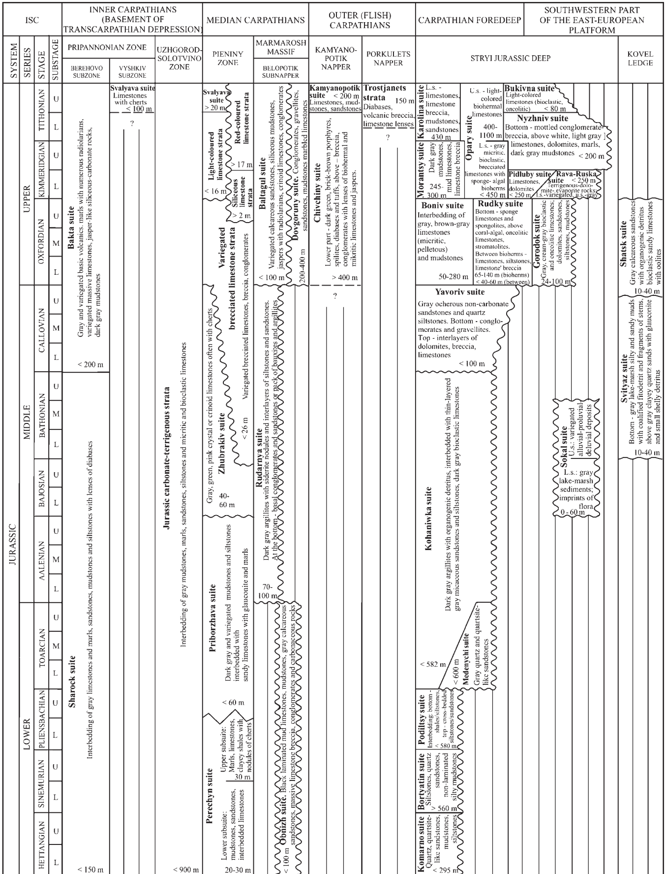
Fig. 2. The Generalized stratigraphic scheme of the Jurassic of the Western Ukraine
