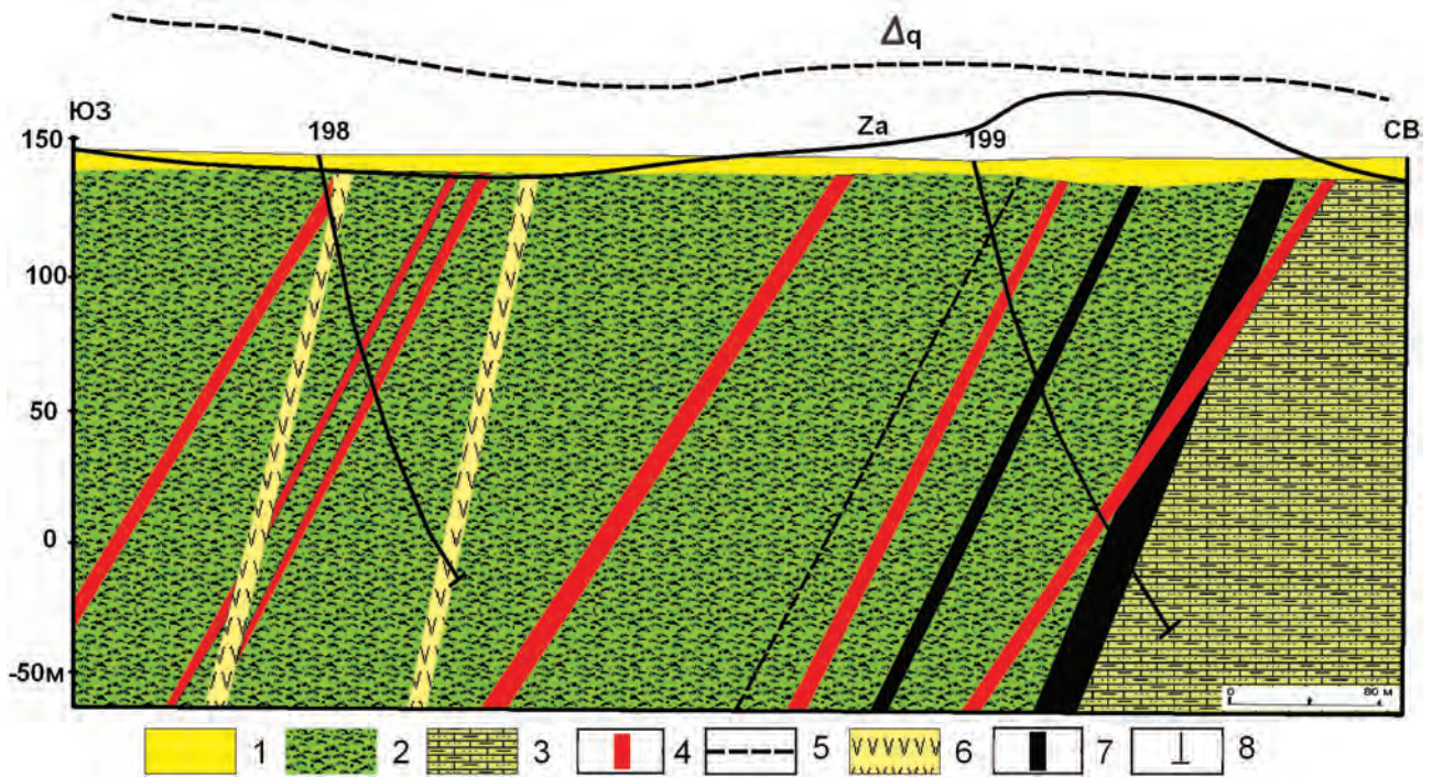
Fig. 2. Fragment of the geological-geophysical section across the strike of the Sorokinskaya trough structure. Compiled by the author on the basis of the materials of Artemovskaya GRE (Н.Ф. Русаков и др., 1981)
