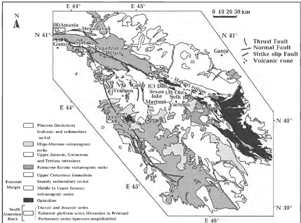
Fig. 1. Geological map of the Lesser Caucasus (after [Sosson et al., 2010], modified), including the location of the key studied areas: A — Old Sotk Pass; B — Amasia; C — Dali.
