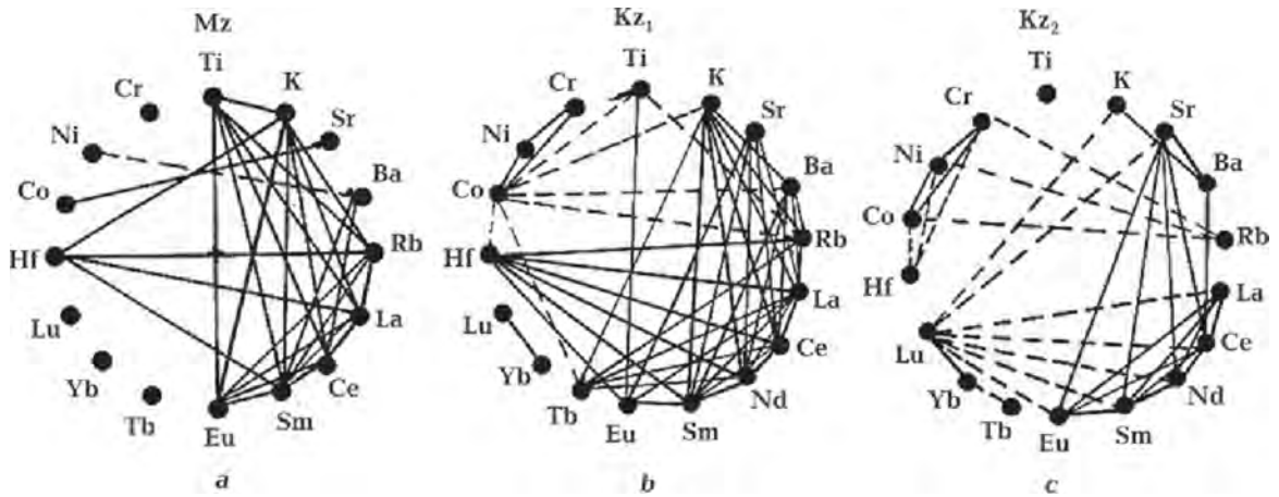
Fig. 5. Correlation of rare elements in Mz (a) and KZ (b, c) in basites of the Lesser Caucasus.
