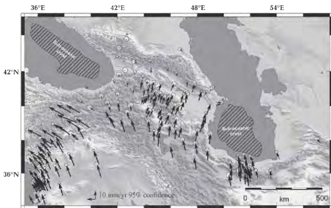
Fig. 1. Map showing global positioning system (GPS) velocities with respect to Eurasia and 95 % confidence ellipses for the eastern Black Sea—Caucasus—Caspian region [Vernant et al., 2013].
