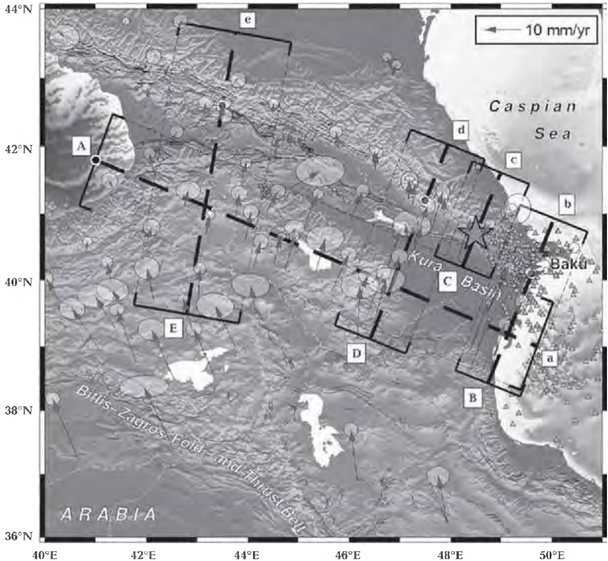
Fig. 1. GPS velocities and 95 % confidence ellipses w.r.t. (with respect to) Eurasia for the eastern AR-EU collision zone.
