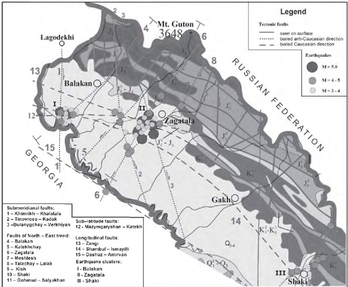
Fig. 1. Allocation of earthquake foci zones of the North-Western Azerbaijan.
