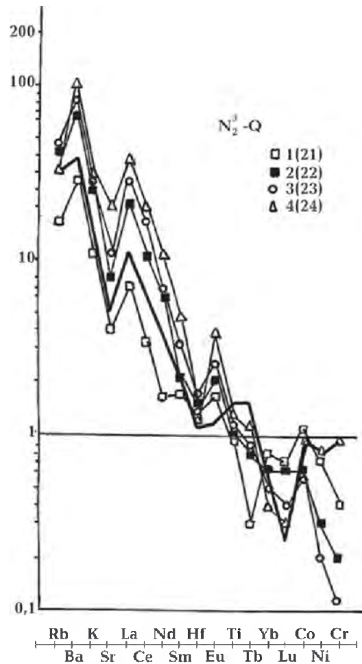
Fig. 4. Normalized multicomponent diagram of the volcanic rock complexes of the Late Pliocene – Holocene: 1 — low potassium dolerite, Trans-Caucasus rise (21); 2 — trachandesibasal, Gegam (22); 3 — trachandesibasal, Kelbajar (23); 4 — basanite, Kafan, Zangezur suture zone (24).
