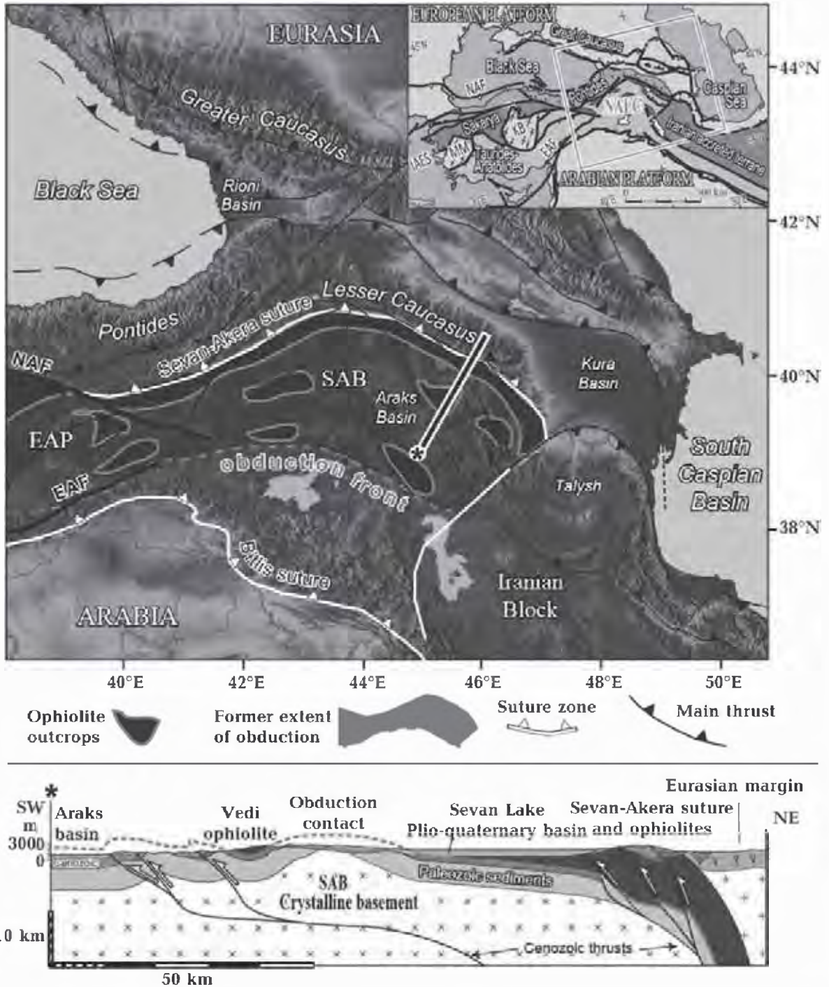
Fig. 1. Tectonic map of the Middle East-Caucasus area, showing the main blocks and suture zones, and corresponding crustal-scale section showing the obduction, after [Hässig et al., 2013]: EAF — East Anatolian Fault; IAES — Izmir—Ankara—Erzincan Suture; KB — Kırsehir Block; MM — Menderes Massif; NALC — North-East Anatolia—Lesser Caucasus domain (zone of ophiolite obduction); SAB — South Armenian Block; V — volcanic arc of Eurasian margin of Pontides. * position of cross-section (below). Lower panel: Upper-crustal-scale geological section of the NALC showing the geometry of the obduction front propagated towards the south and its rooting into the Sevan Akera suture to the north, below the Eurasian margin (see [Rolland et al., 2012]).
