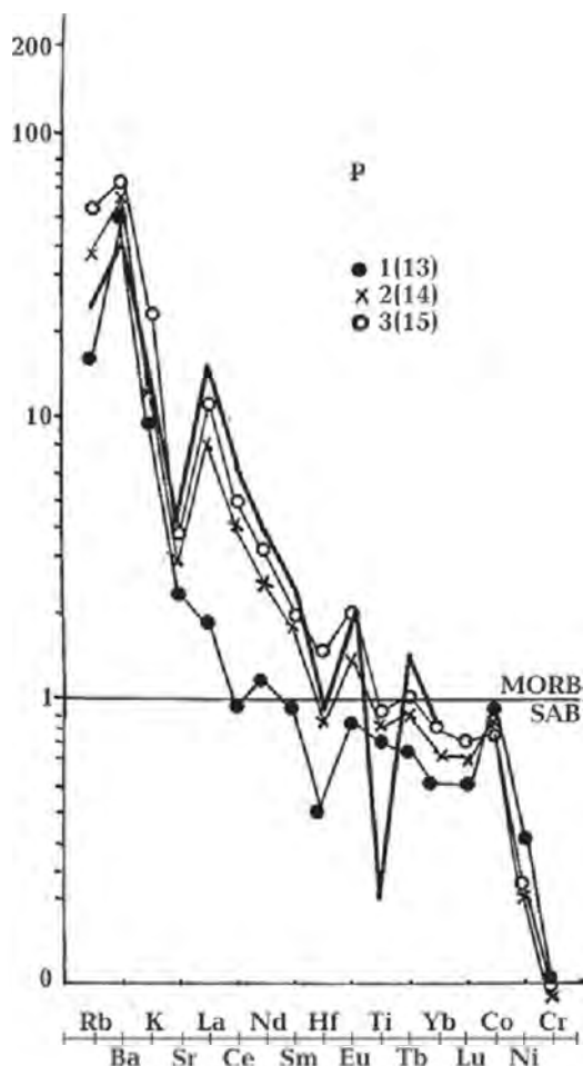
Fig. 1. Normalized multicomponent diagram of the volcanic rock complexes of the Middle Eocene (Yerevan-Ordubad zone): 1 — toleitic basalt (13); 2 — calc-alkaline basalt (14); 3 — Trakhibasalt (15).
