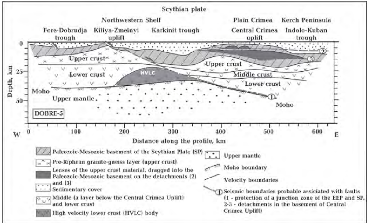
Fig. 1. Interpreted seismic model on the DOBRE-5 profile.
