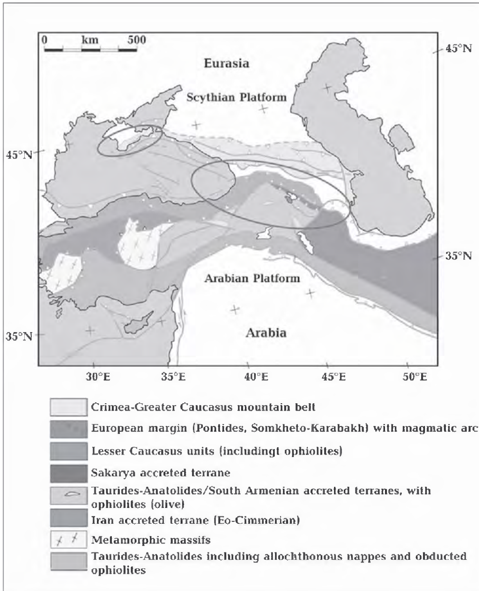
Fig. 1. Tectonic map of the Black Sea-Caucasus domain and surrounding areas, modified from [Sosson et al., 2016, 2017], showing the main field locations of IRG studies.
