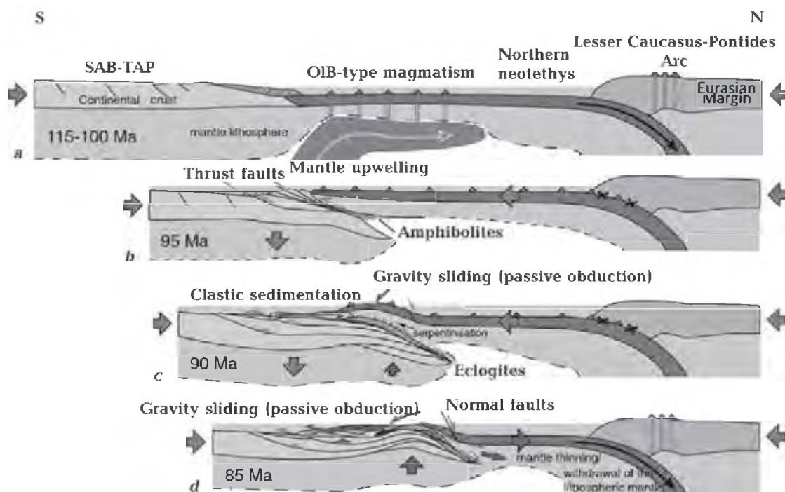
Fig. 2. Conceptual model of the obduction process in the NALC: a — situation in the Early Cretaceous showing the convergence of SAB—TAP (South Armenian Block—Taurides Anatolides) with the Eurasian margin, the onset of mantle upwelling and heating of the oceanic lithosphere at 115 Ma, b — triggering of obduction, due to the blocking of the northern subduction zone and the increase in buoyancy of the oceanic lithosphere, c — thickening of the continental crust below the obduction, erosion and the onset of passive obduction [Lagabrielle et al., 2013] by gravity sliding of the ophiolites on the flexural basin, d — transition from a contractional to an extensional regime due to renewed subduction. Mantle thinning and withdrawal leads to the exhumation of the continental crust.
