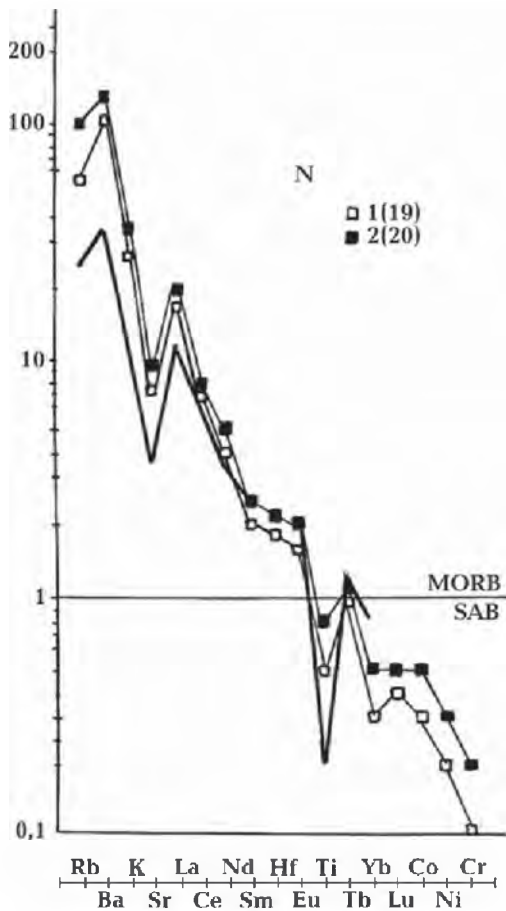
Fig. 3. Normalized multicomponent diagram of the volcanic rock complexes of the Neogene (Yerevan-Ordubad zone): 1 — andesite (19); 2 — andesite (20).
