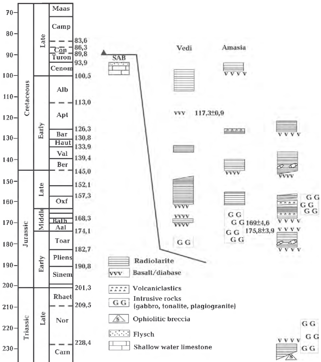
Fig. 2. Synthesis of all known ages (both biochronological and geochronological) for the ophiolitic rocks and their sedimentary cover in the Lesser Caucasus (after [Danelian et al., 2016], modified).
