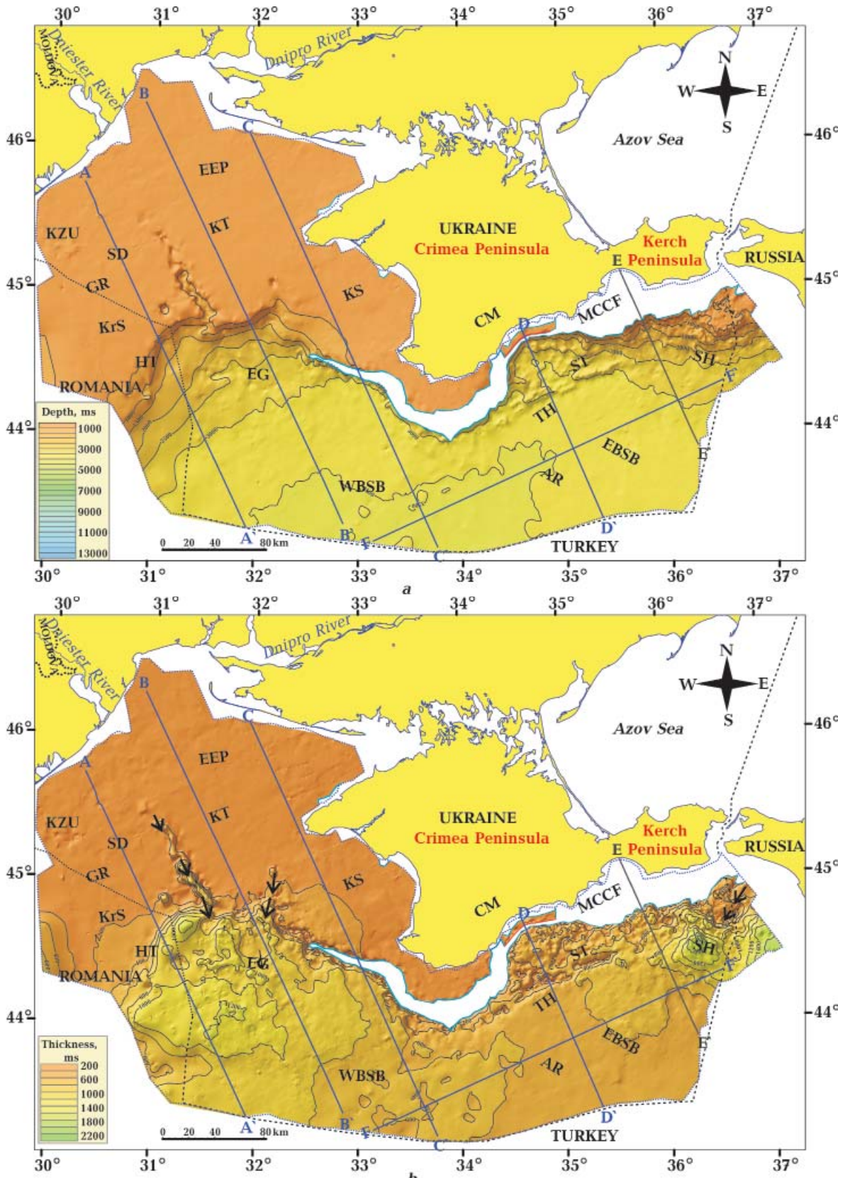
Fig. 20. TWT structural map at the base of the Quaternary sediments (a) and TWT thickness map of the Quaternary sequence (b) for the study area. The black arrows in (b) show valleys of paleo-rivers. See Fig. 2 for abbreviations of tectonic units and Fig. 9 for other explanations and abbreviations.
