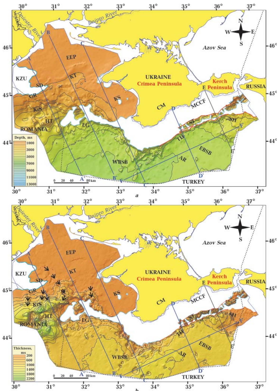
Fig. 18. TWT structural map at the base of the upper part of the Pontian sediments (Messinian unconformity?), the Upper Miocene (a) and TWT thickness map of the upper part of the Pontian sequence (b) for the study area. The black arrows in (b) show valleys of paleo-rivers. See Fig. 2 for abbreviations of tectonic units and Fig. 9 for other explanations and abbreviations.
