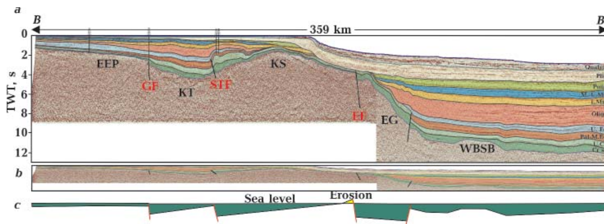
Fig. 4. Interpreted seismic reflection profile B—B'. See Fig. 3 for explanation; see also Fig. 2 for abbreviations of regional tectonic units and Fig. 3 for abbreviations of sedimentary sequences. Abbreviations of fault names (in red): GF — Golitsin Fault; EF — Euxinian Fault; STF — Sulina—Tarkhankut Fault.
