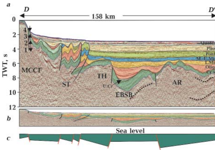
Fig. 6. Interpreted seismic reflection profile D—D'. See Fig. 3 for explanation; see also Figs. 2—3 for abbreviations of regional tectonic units and sedimentary sequences. Black arrows show directions of movements of the hanging wall at the present-day continental slope during: 1 — Cretaceous rifting; 2 — Eocene compression; 3 — Late Miocene compressions; 4 — Quaternary extension. The dotted lines beneath the Cretaceous syn-rift sequence correspond to horizons illuminating the structure of pre-rift sediments in the EBSB and Andrusov Ridge.
