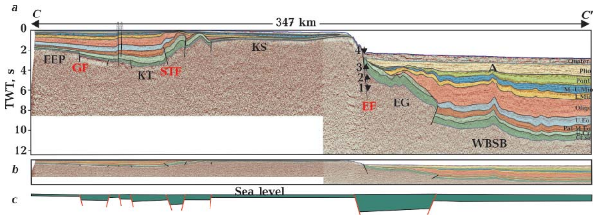
Fig. 5. Interpreted seismic reflection profile C—C'. See Fig. 3 for explanation; see also Figs. 2—4 for abbreviations of regional tectonic units, faults and sedimentary sequences. Black arrows show directions of movements of the EF hanging wall during: 1 — Cretaceous rifting; 2 — Eocene compression; 3 — Late Miocene compressions; 4 — Quaternary extension. The anticline labelled «A» is a local structure that was formed in the WBSB under submarine conditions during the Late Miocene compression events.
