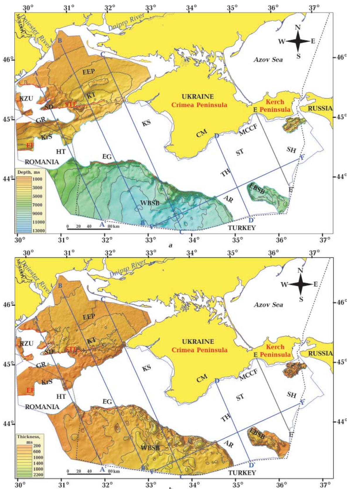
Fig. 14. TWT structural map at the base of the Upper Eocene sediments (a) and TWT thickness map of the Upper Eocene sequence (b) for the study area. See Fig. 2 for abbreviations of tectonic units and Fig. 9 for other explanations and abbreviations.
