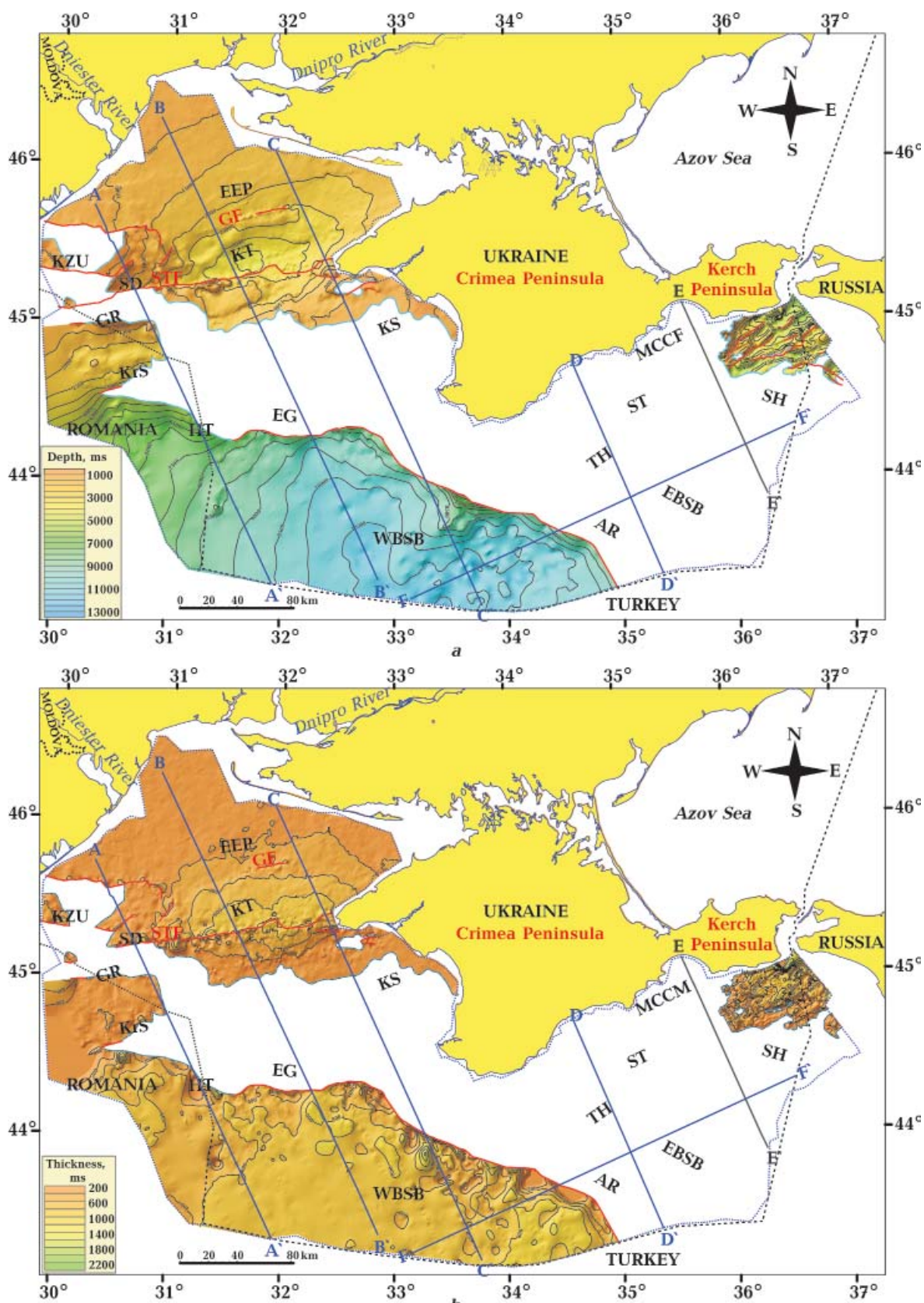
Fig. 12. TWT structural map at the base of the Paleocene-Middle Eocene post-rift sediments (a) and TWT thickness map of the Paleocene—Middle Eocene post-rift sequence (b) for the study area. See Fig. 2 for abbreviations of tectonic units and Fig. 9 for other explanations and abbreviations.
