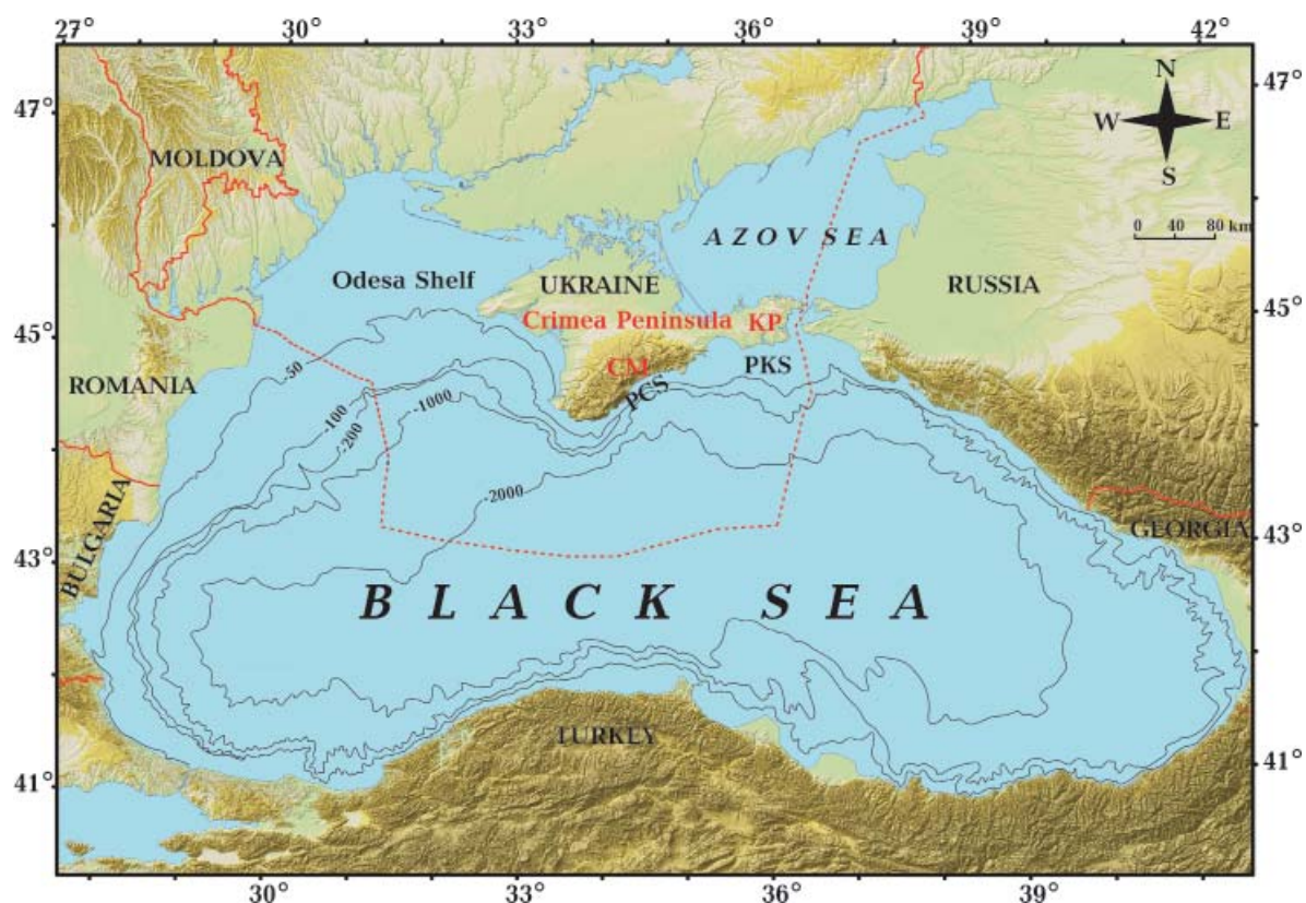
Fig. 1. Physiographic map of the Black Sea region. Red lines are country boundaries; red dashed line is the boundary of the Ukrainian sector of the Black Sea and Azov Sea. Abbreviations: CM — Crimean Mountains; KP — Kerch Peninsula; PCS — Pre-Crimea Shelf; PKS — Pre-Kerch Shelf.
