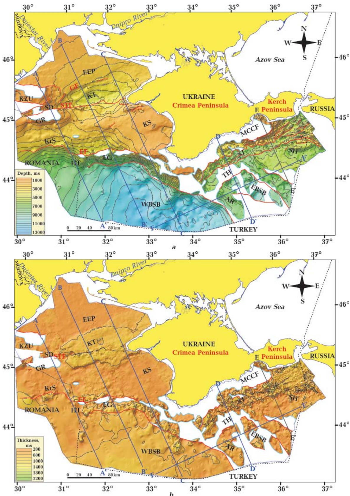
Fig. 11. TWT structural map at the base of the Upper Cretaceous post-rift sediments (a) and TWT thickness map of the Upper Cretaceous post-rift sequence (b) for the study area. See Fig. 2 for abbreviations of tectonic units and Fig. 9 for other explanations and abbreviations.
