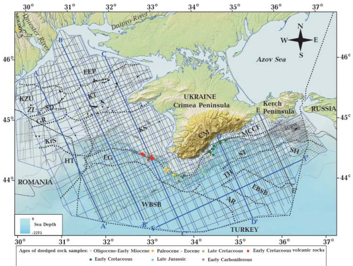
Fig. 2. Physiographic map of the study area and contours of regional tectonic units (in black bold dotted lines), locations of key offshore wells (black dots), interpreted seismic reflections profiles (grey and blue lines), locations and ages of rock samples dredged from the sea bottom (colour dots). The regional seismic lines conducted in the framework of BS05 and UBS94 projects are shown in blue and grey lines respectively; seismic lines of other 2D seismic surveys are shown with grey dashed lines. The area of seismic study is shown with blue dashed line. The black dashed line is the limit of the Ukrainian sector of the Black Sea. The seismic profiles shown in Figs 3—8 are in blue and grey bold lines. Abbreviations of tectonic units and wells: AR — Andrusov Ridge; CM — Crimean Mountains; EBSB — Eastern Black Sea Basin; EEP — Eastern European Platform; EG — Euxinian Graben; GR — Gubkin Ridge; HT — Histria Trough; KrS — Krayova Step; KS — Kalamit Swell; KT — Karkinit Trough; KZU — Krylov-Zmiiny Uplift; MCCF — the Marine Continuation of the Crimean Folds; SD — Sulina Depression; SH — Shatskiy High; ST — Sorokin Trough; SUBW — Subbotina wells; TH — Tetyaev High; WBSB — Western Black Sea Basin; ZI — Zmiiny Island, coincident with the location of the Morskaya-1 well (black dot).
