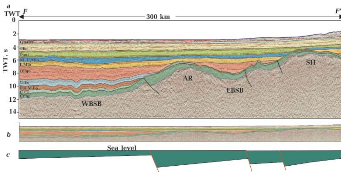
Fig. 8. Interpreted seismic reflection profile F—F'. See Fig. 3 for explanation; see also Figs. 2, 3 for abbreviations of regional tectonic units and sedimentary sequences.
