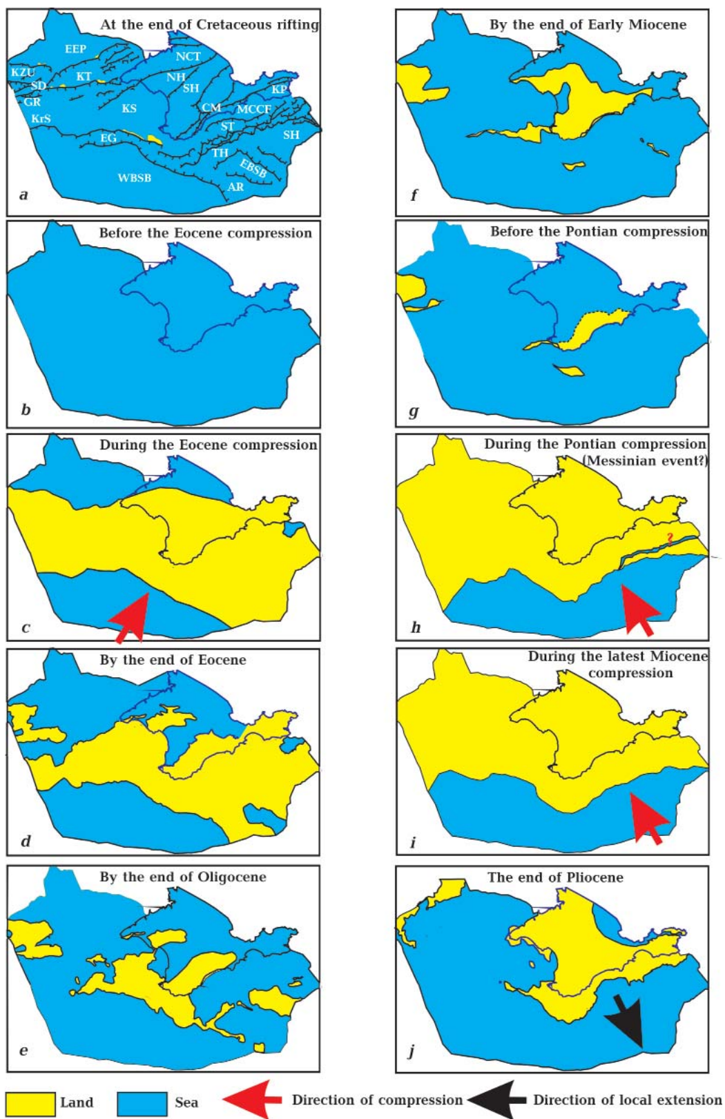
Fig. 13. Simplified paleotectonic reconstructions demonstrating the distribution of offshore and onshore areas for ten time slices. The data on the Crimea Peninsula are adopted from [Stovba et al., 2017a,b]. Abbreviations of present-day regional tectonic units: KP — Kerch Peninsula; NCT — North-Crimea Trough; NH — Novoselivka High; SH — Simferopol High. See Fig. 2 for other abbreviations.
