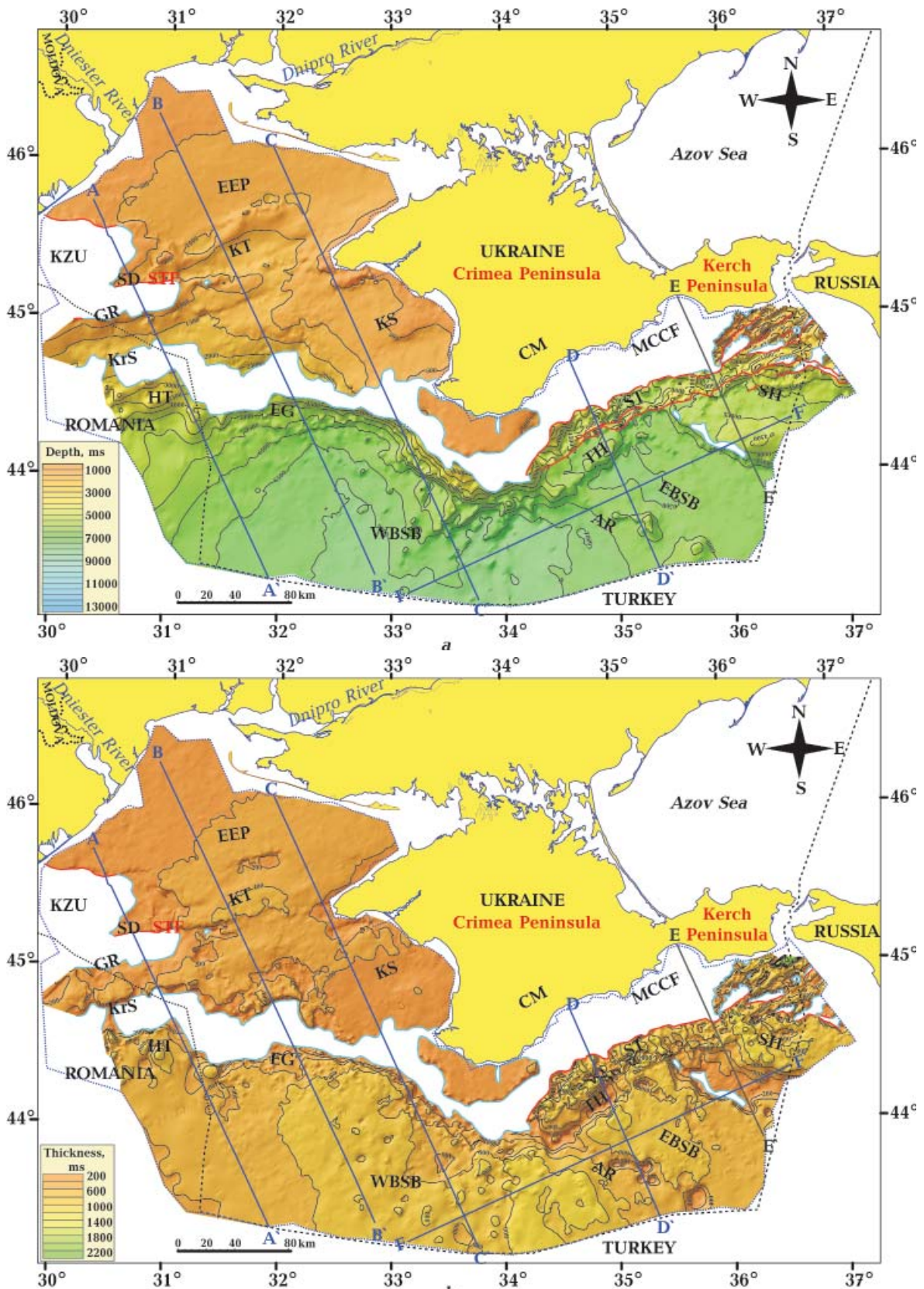
Fig. 16. TWT structural map at the base of the Lower Miocene (upper part of Maykopian) sediments (a) and TWT thickness map of the Lower Miocene sequence (b) for the study area. See Fig. 2 for abbreviations of tectonic units and Fig. 9 for other explanations and abbreviations.
