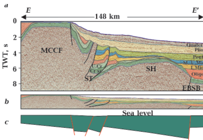
Fig. 7. Interpreted seismic reflection profile E—E'. See Fig. 3 for explanation; see also Figs. 2—3 for abbreviations of regional tectonic units and sedimentary sequences.
