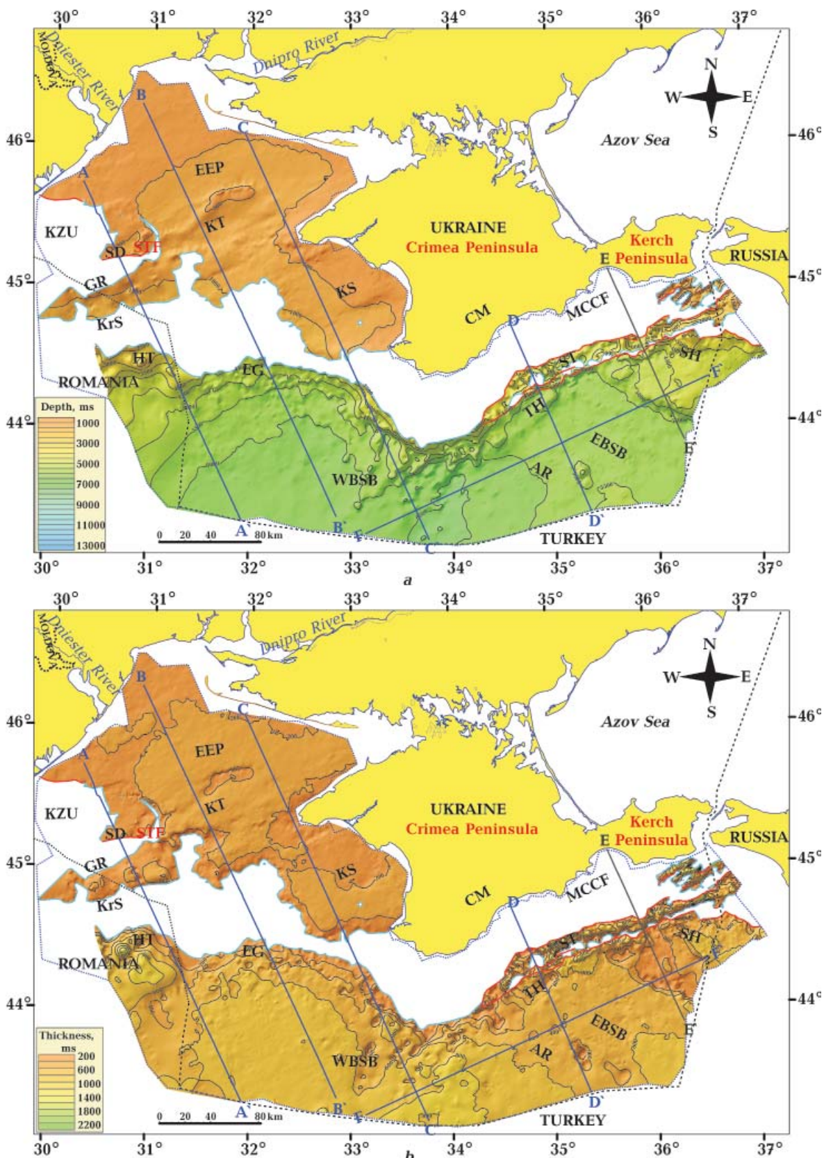
Fig. 17. TWT structural map at the base of the Middle-Late Miocene sediments (a) and TWT thickness map of the Middle-Late Miocene sequence (b) for the study area. See Fig. 2 for abbreviations of tectonic units and Fig. 9 for other explanations and abbreviations.
