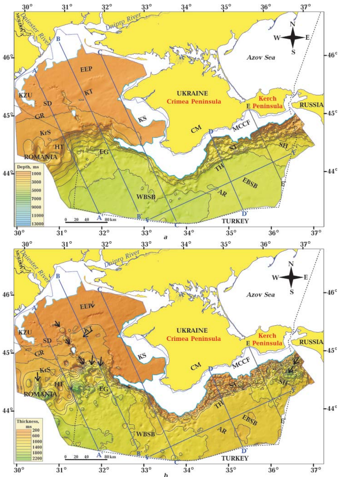
Fig. 19. TWT structural map at the base of the Pliocene sediments (a) and TWT thickness map of the Pliocene sequence (b) for the study area. The black arrows in (b) show valleys of paleo-rivers. See Fig. 2 for abbreviations of tectonic units and Fig. 9 for other explanations and abbreviations.
