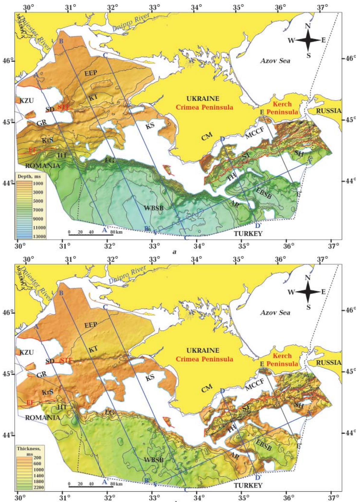
Fig. 15. TWT structural map at the base of the Oligocene (lower part of Maykopian) sediments (a) and TWT thickness map of the Oligocene sequence (b) for the study area. See Fig. 2 for abbreviations of tectonic units and Fig. 9 for other explanations and abbreviations.
