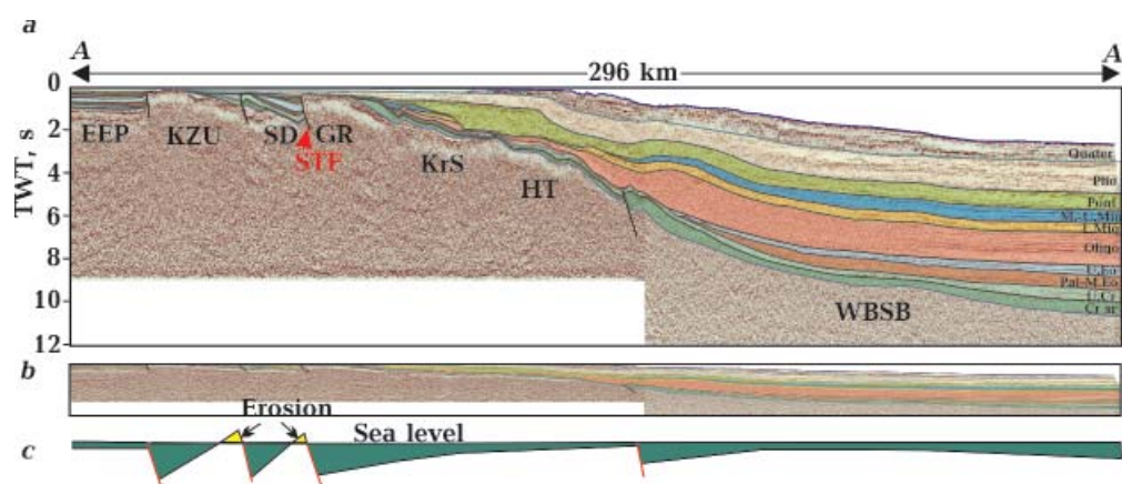
Fig. 3. Interpreted seismic reflection profile A—A' (a); the same profile with vertical scale reduced in 5 times is shown in (b). A simplified paleotectonic reconstruction of basin structure along the profile during Cretaceous rifting is demonstrated in (c); no depth scale is applicable for the reconstruction. The location of the profile is shown in Fig. 2. Quater — Quaternary; Plio — Pliocene; Pont — middle and upper Pontian; M.-U.Mio — Middle and Upper Miocene; L.Mio — Lower Miocene (upper part of Maykopian sediments); Oligo — Oligocene (lower part of Maykopian sediments); U.Eo — Upper Eocene; Pal.-M.Eo — Paleocene—Middle Eocene; U.Cr — post-rift Upper Cretaceous; Cr sr — Lower and Upper Cretaceous syn-rift sediments. STF — Sulina-Tarkhankut Fault. The abbreviations for the tectonic units are described in Fig. 2.
