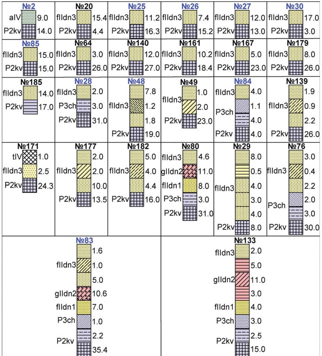
Fig. 2. Geological-lithological columns by wells.
