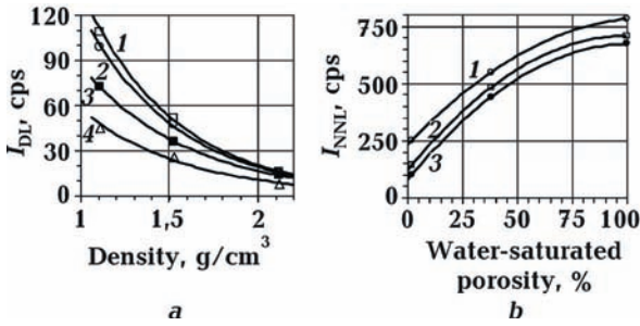
Fig. 5. Dependencies of readings on discrimination level (millivolt): a — for DL-channel (1 — 100, 2 — 300, 3 — 400, 4 — 500); b — for near detector of 2NNL-tool (1 — 35, 2 — 55, 3 — 70).
