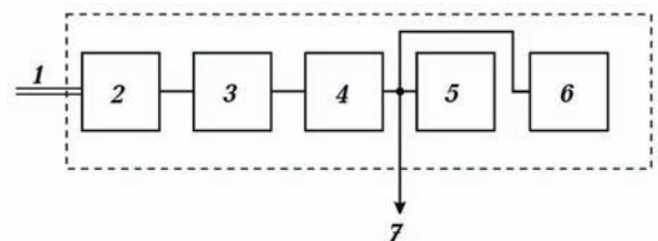
Fig. 4. Block scheme of console: 1 — connection of logging cable with console, 2 — amplifier, 3 — discriminator, 4 — microprocessor, 5 — flash memory, 6 — numeric display, 7 — output to computer.
