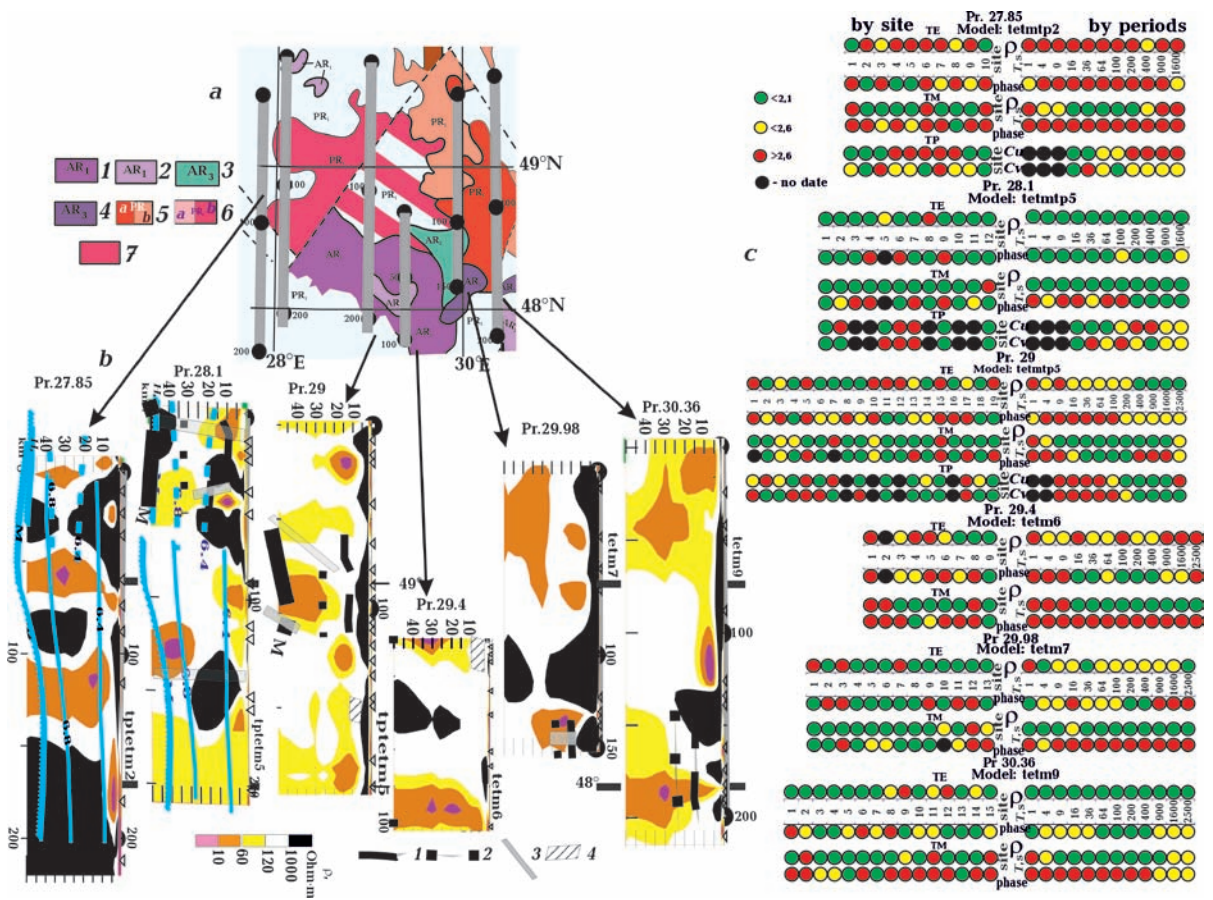
Fig. 2. Geological map of pre-Riphean deposits [National..., 2007] (a): 1 — enderbites; 2 — gneisses, crystal-line schists, amphibolites, calciphyres, ferruginous quartzites, mafic rocks, ultramafic rocks; 3 — plagiogranites, diorites, granodiorites, gneisses, amphibolites, marbles, crystalline schists, marbles, crystalline schists, gneisses, amphibolites; 4 — gneisses, ferruginous quartzites, marbles, crystalline schists, gneisses, amphibolites, pyroxenites; 5 — granites (a), migmatites (b); 6 — granites, migmatites (a), charnockites (b); 7 — granites, migmatites, granodiorites, diorites. Geoelectric models along meridional profiles with the best RMS. Seismogeological sections along geotraverses EUROBRIDGE (dashed line); Bucharest—Chornobyl (solid) and YI (see Fig. 1) (b): 1, 2 — velocity contours: V_p = 6.4 km/s (1), V_p = 6.8 km/s (2), 3 — fault lines; 4 — low velocity zones. Residuals (RMS) in experimental and model data (c).
