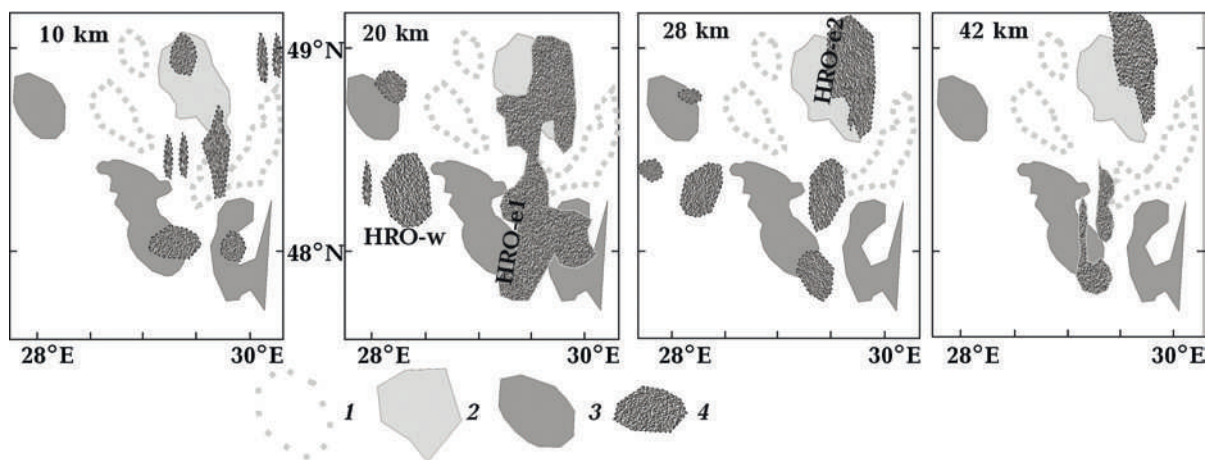
Fig. 11. Comparison of Bouguer anomaly values [National..., 2007]: 1 — 10 mGal, 2 — more than 20 mGal, 3 — more than 30 mGal, 4 — with rock distribution with r values of more than 4000 Ohm·m. HRO — high blocks stretching to great depths (see Fig. 4).
