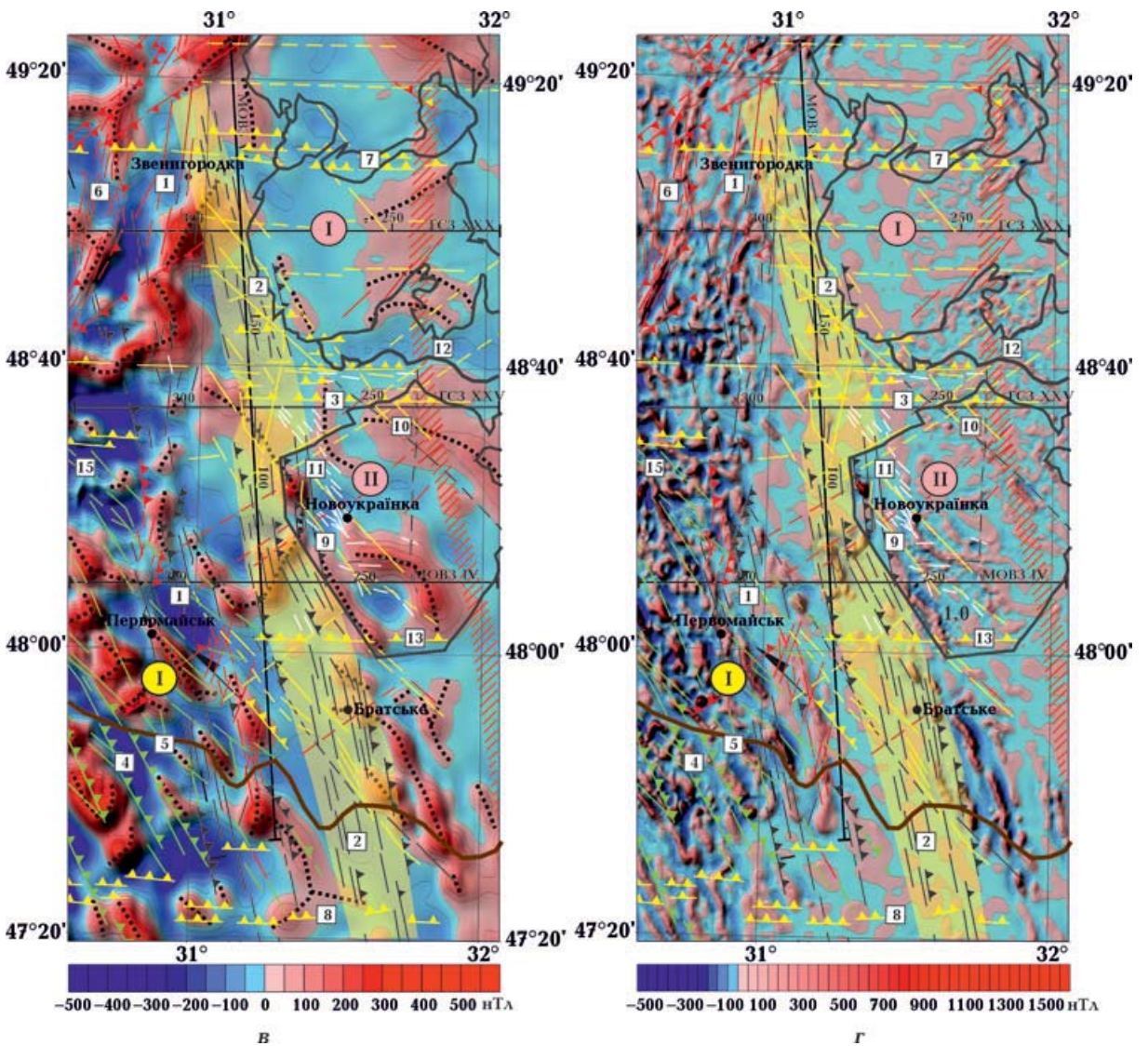
Fig. 2. Maps of anomalous magnetic field components: regional (\Delta B)_{a, \text{per.}} (a), local (\Delta B)_{a, \text{lok.}} (b), local «medium wave» (\Delta B)_{a, \text{lok. cx.}} (c), local «short-wave» (\Delta B)_{a, \text{lok. kx.}} (d). Regional magnetic anomalies (numbers in circles): 1 — Kyivs'ka, 2 — Haysyns'ka, 3 — Ananiivs'ka, black dashed lines — axes of magnetic anomalies. For whole legend, see Fig. 1.
