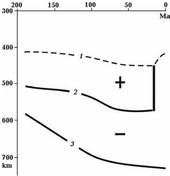
Fig. 7. Zones of rock volume changes under the influence of polymorphic transitions in the considered region: 1 — depth of the start of the Ol\alpha \leftrightarrow Ol\beta transition, 2 — the boundary of the change in the sign of the temperature change with time, 3 — the boundary of zero temperature changes or the surface of the global asthenosphere; + and — are zones of expansion and compression of rocks.
