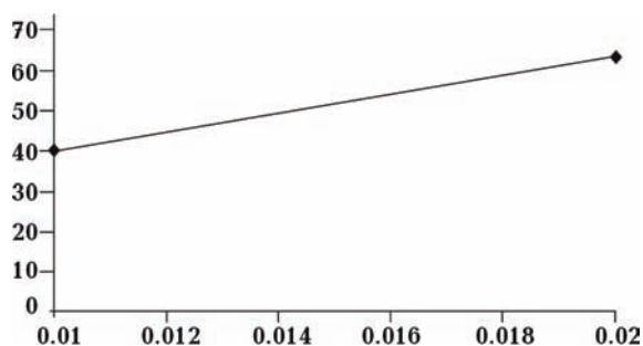
Fig. 4. Plot of relation between well production and conventional coefficient of absorption. Axis Y — gas production volume, thousands m^3/day , axis X — absorption, conventional units, well 12, well 403 (well 12 at the beginning of the figure).
