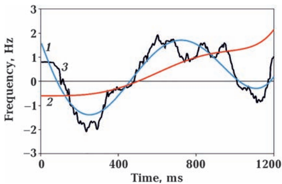
Fig. 3. Unconstrained (1) and constrained (2) polynomials approximating \Delta\bar{\omega}(t) (3).
