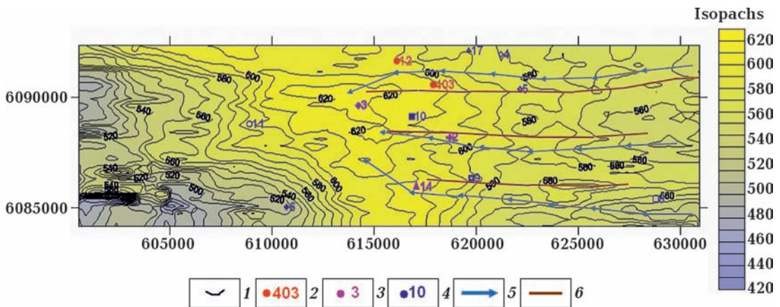
Fig. 9. Thickness map of the Late Serpukhovian substage: 1 — iso-pachous line of Late Serpukhovian substage sediments; 2 — producing wells within horizon C-1; 3 — producing wells within horizon C-2; 4 — barren wells within Late Serpukhovian; 5 — line of thalwegs; 6 — line of interstream areas. Axes Y and X — conventional geographic coordinates. Structural complications in the lower left corner are caused by the presence of the South Pereshchepino stock.
