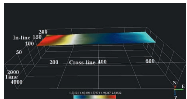
Fig. 7. Seismic reflector in the bottom of the Bashkirian substage (by OpendTect).
