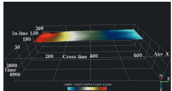
Fig. 6. Seismic reflector in the bottom of the Late Serpukhovian substage (by OpendTect).
