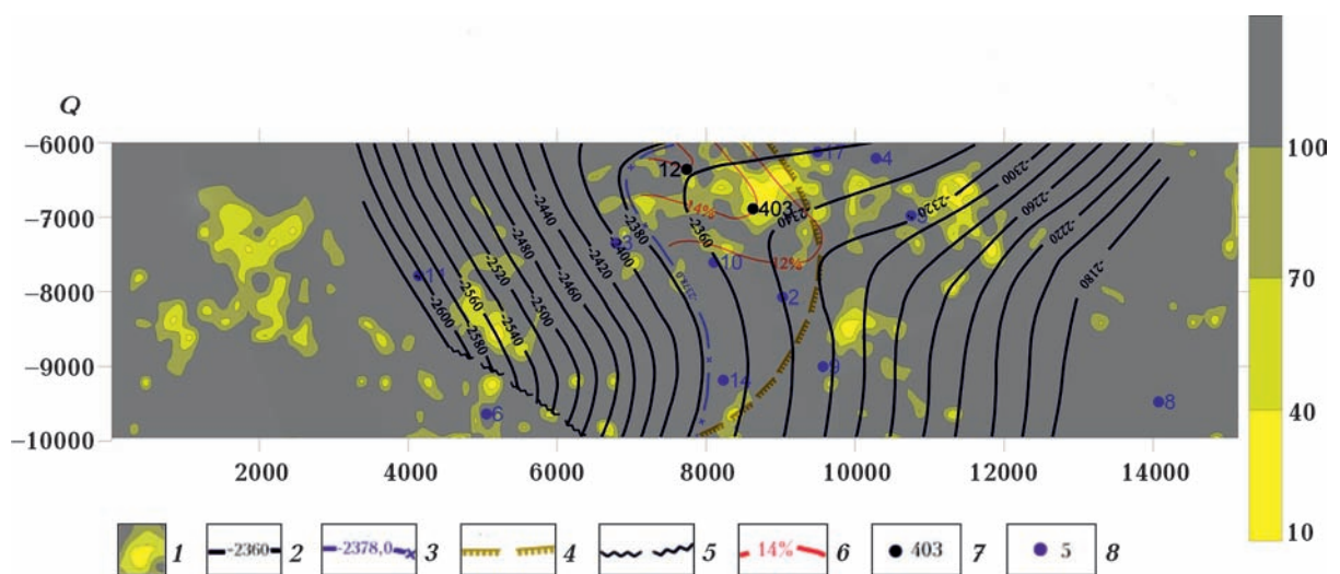
Fig. 1. Map of medium Q changing along horizon C-1 within the Bogatoika area: 1 — changes of parameter Q , 2 — contour line of roof of productive horizon C-1, 3 — contour line of gas-water surface, 4 — line of lithological replacement of a reservoir, 5 — boundary line of horizon washout, 6 — contour line of equal values of porosity, 7 — producing well, 8 — barren well.
