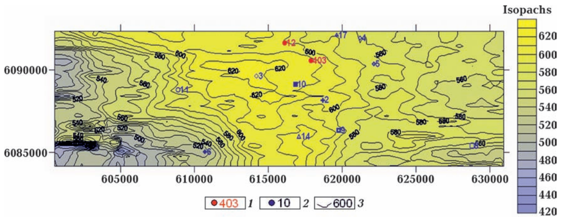
Fig. 8. Thickness map of the Late Serpukhovian substage: 1 — producing well within horizon C-1; 2 — barren well within horizon C-1; 3 — lines of thickness equal meanings of the Late Serpukhovian substage. Axes Y and X — conventional geographic coordinates. Structural complications in the lower left corner are caused by presence of the South Pereshchepino salt stock.
