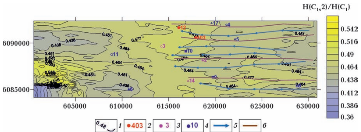
Fig. 10. Ratio map of thicknesses of the Late Serpukhovian substage to all Serpukhovian: 1 — ratio line of thicknesses of the Late Serpukhovian substage to the whole Serpukhovian; 2 — producing wells within horizon C-1; 3 — producing wells within horizon C-2; 4 — barren wells within Late Serpukhovian; 5 — line of thalwegs; 6 — line of interstream areas. Structural complications in the lower left corner of the map are caused by the presence of the South Pereshchepino stock.
