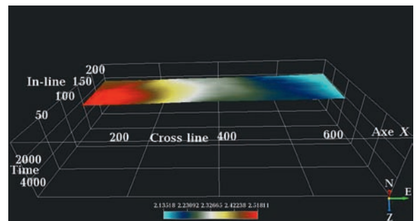
Fig. 5. Seismic reflector in the bottom of the Early Serpukhovian substage (by OpendTect).
