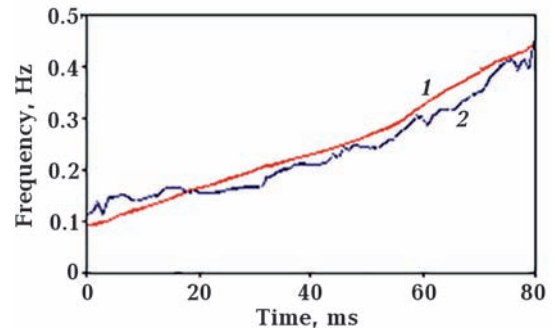
Fig. 2. Estimations of \Delta\bar{\omega}(t) obtained with (1) and without (2) introducing weighting function \omega(t) .
