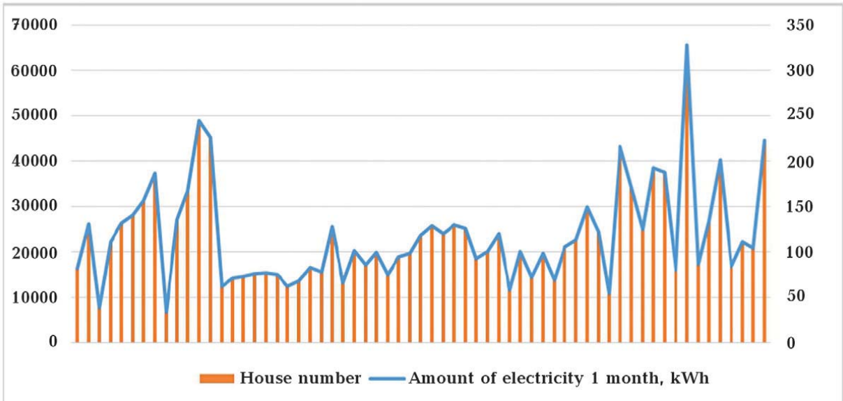
Fig. 12. Graph of the dependence of the calculated amount of energy on the number of houses in the Begimdag-Tekchai zone.
