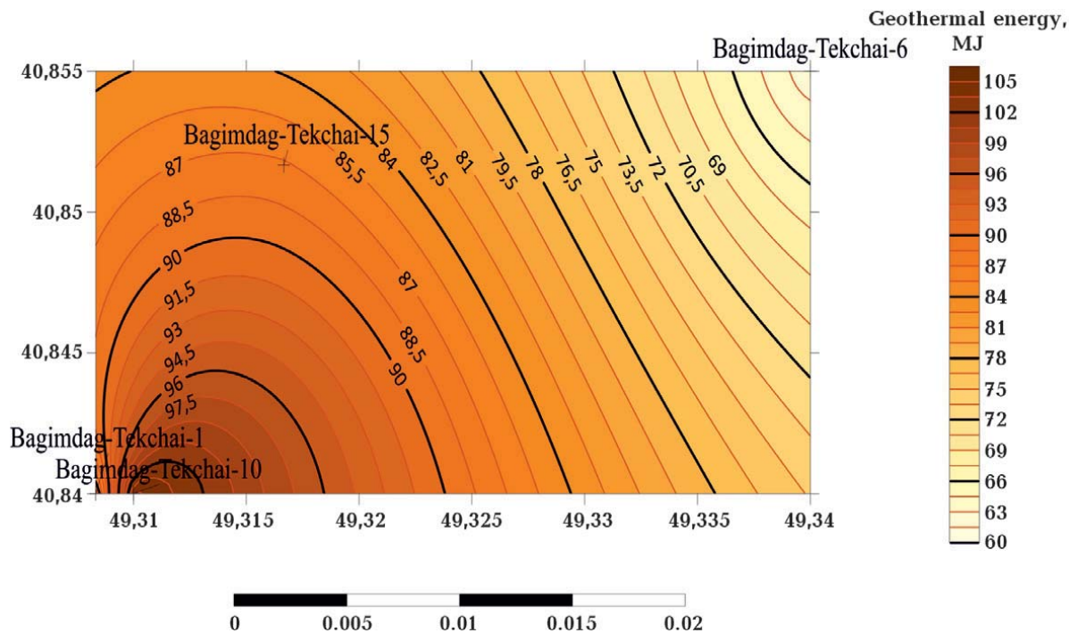
Fig. 11. Distribution map of calculated energy potential for wells 1, 6, 10 of the Begimdag-Tekchai field.
