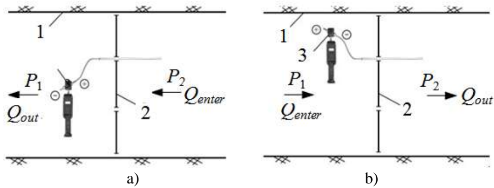
1 – mine working; 2 – ventilation structure; 3 – pressure difference converter
