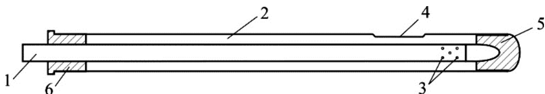
1 – measuring tube; 2 – protective tube; 3 – measuring holes of the measuring tube; 4 – the entrance hole of the protective tube; 5 - stopper; 6 – plug-stopper
