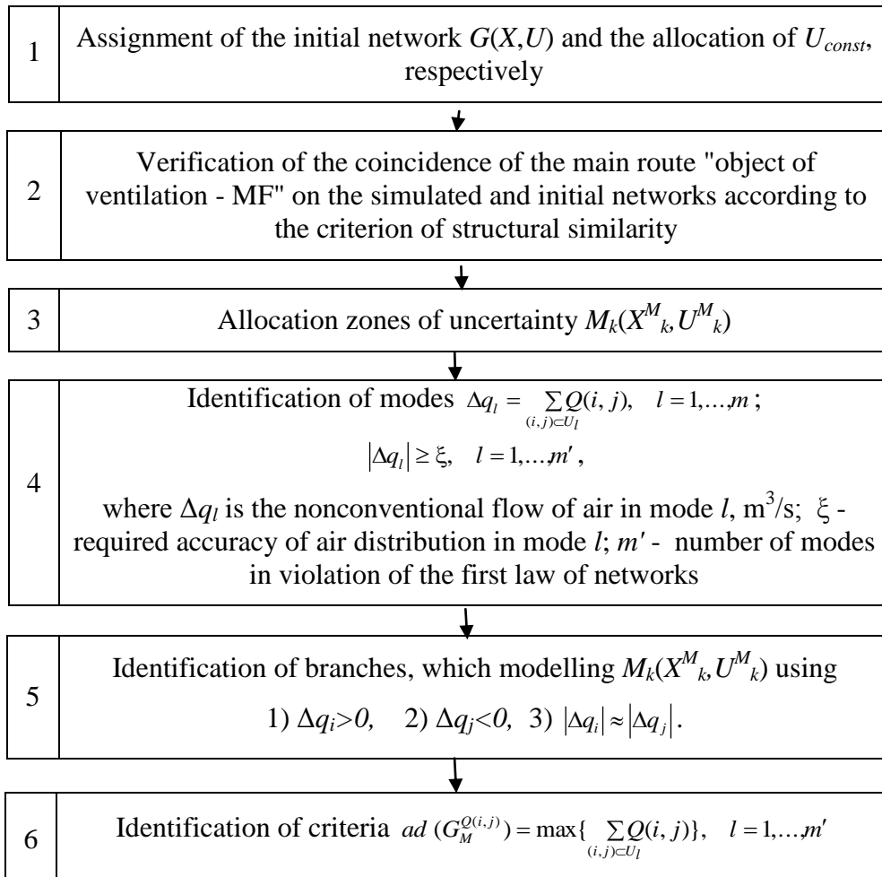
Figure 2 - Algorithm for structural identification of MVN
