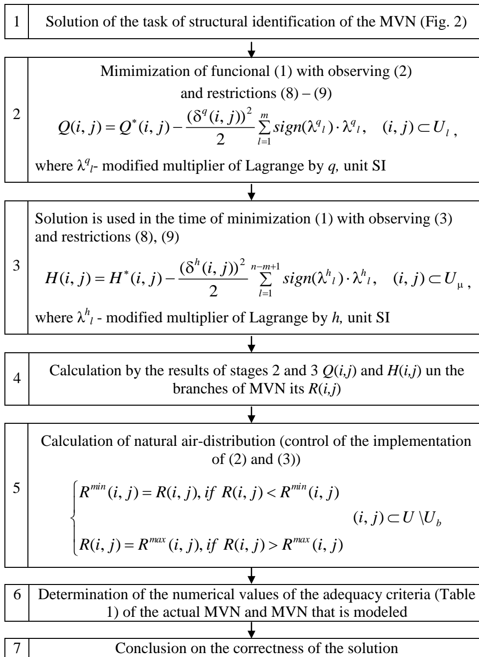
Figure 3 - Algorithm of parametrical identification of the MVN
