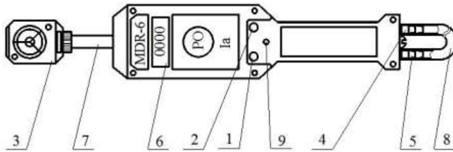
1 – button to switch to the mode of measurement of pressure differences; 2 – the power button in the mode measurements of temperature and air humidity; 3 – remote sensor of temperature and humidity of the environment; 4 and 5 – pressure pipes; 6 – digital indicator; 7 – telescopic lengthening; 8 – preventive tube; 9 – checkpoint
