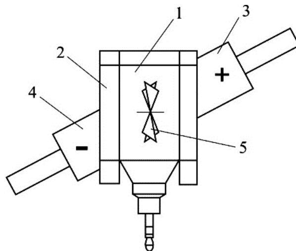
1 – the primary converter of the air velocity of the anemometer APR-2; 2 – lid; 3 – high-pressure nozzle; 4 – low pressure nozzle; 5 – impeller
