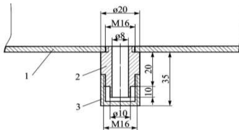
1 – pipeline; 2 – carbine; 3 – protective hubcap
