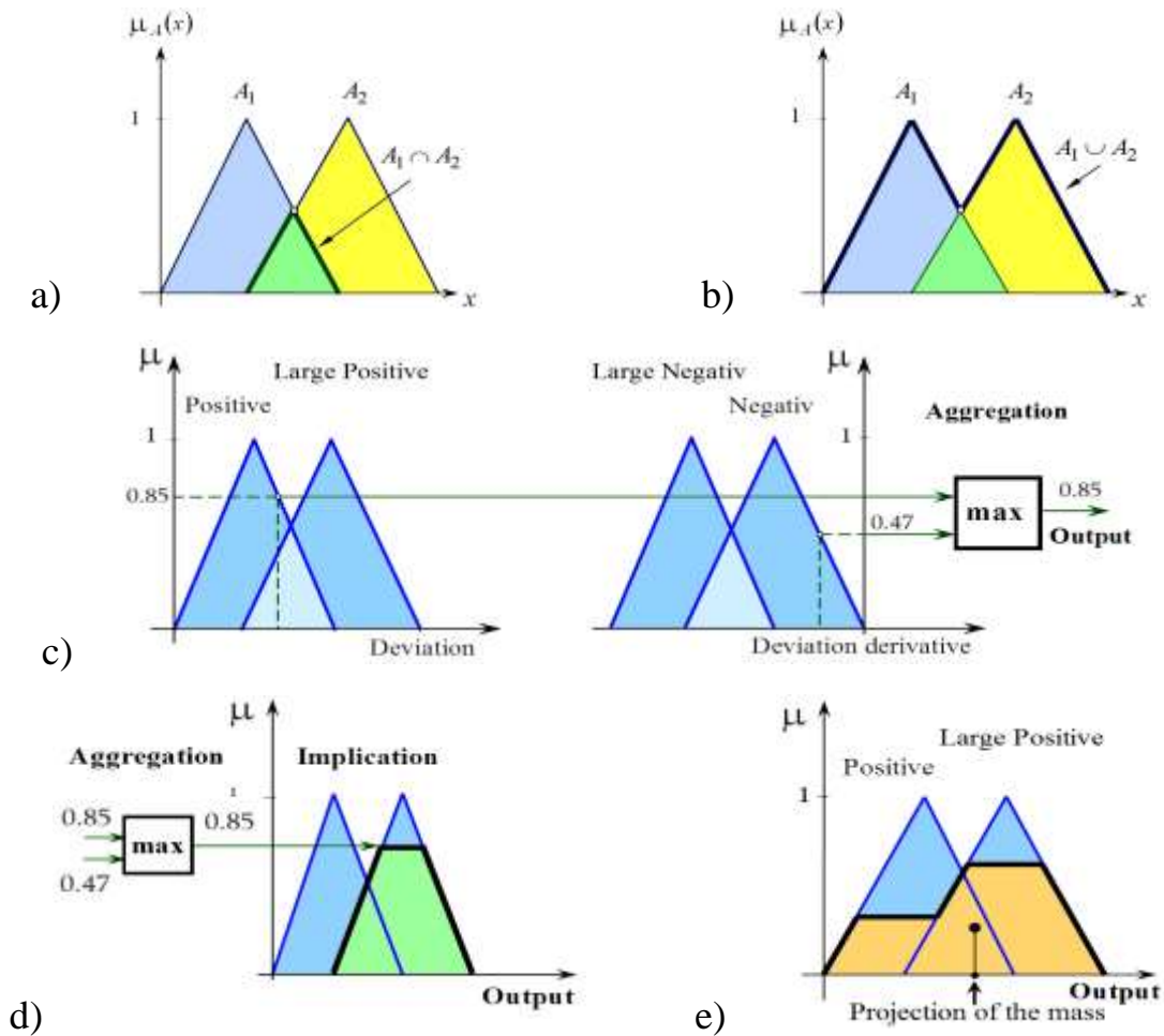
Figure 2 – Methods of calculations used in fuzzy controller: intersection (a) and union (b) of fuzzy sets, aggregation processes (c) and implication (d), defuzzification of the result of calculations (e)
