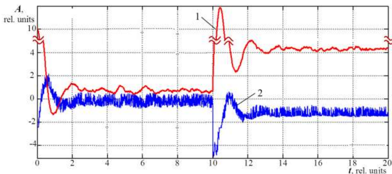
Figure 3 – Modeling fuzzy regulator: 1 – the output signal of the conventional regulator; 2 – correction signal of the fuzzy regulator “Output”.
