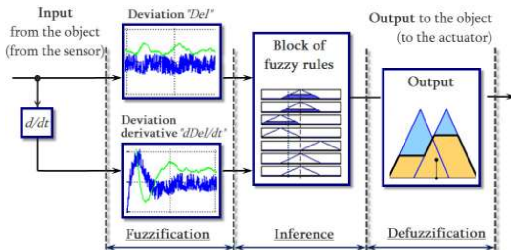
Figure 1 – The signal processing circuit in fuzzy controller
