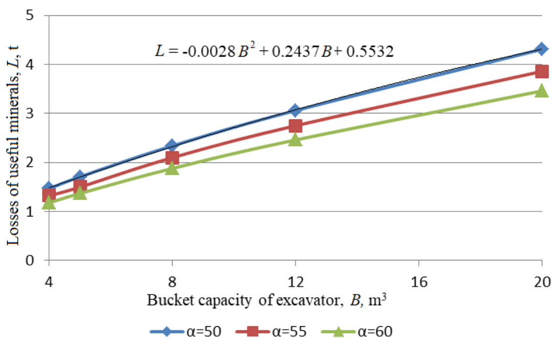
Figure 1 - Dependence of ore losses upon bucket capacity
