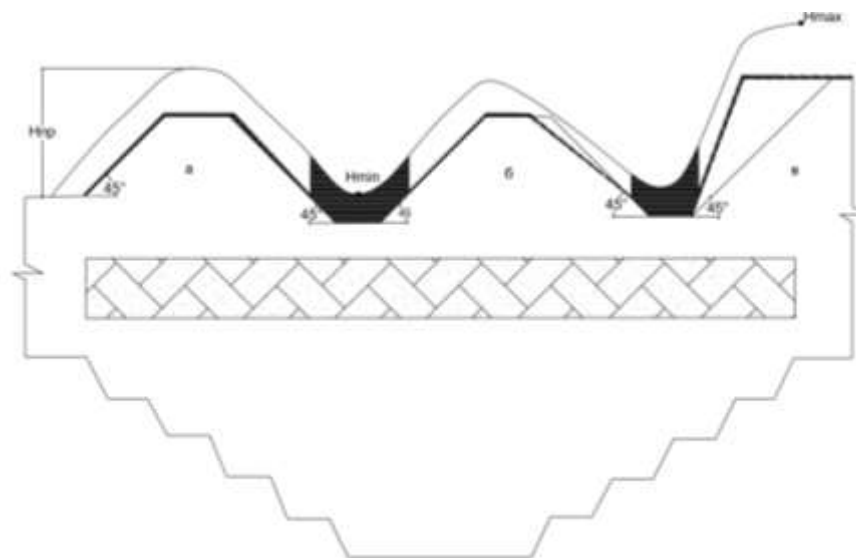
Figure 4 – Scheme of stage-by-stage mesorelief formation
