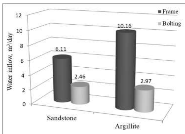
Figure 6 – Changing the values of water inflow into mine working with frame and roof-bolting fastening in rocks with different water stability
