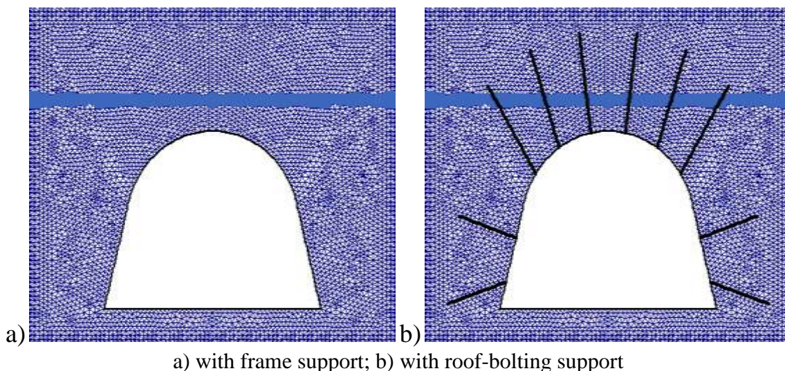
Figure 1 – The central fragment of the finite element grid, the water bearing coal interlayer above the mine working
