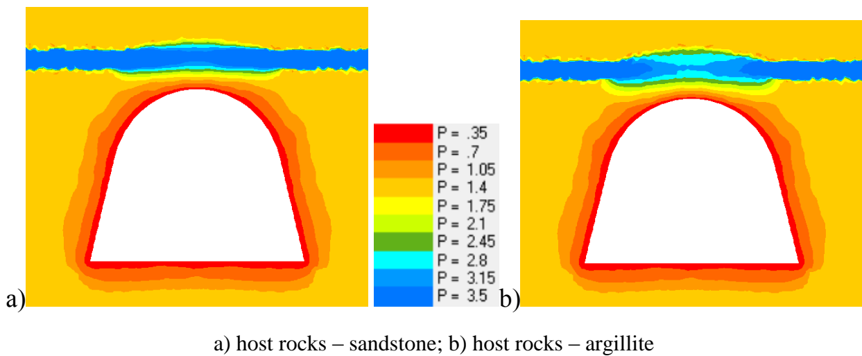
Figure 4 – The distributions of water pressure values, MPa, in mine working with frame support
