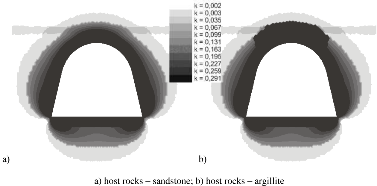
Figure 2 – The distributions of permeability coefficients values of the rocks around mine working with frame support
