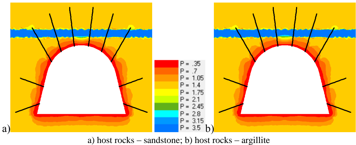
Figure 5 – The distributions of water pressure values, MPa, in mine working with roof-bolting support
