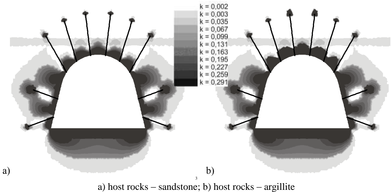
Figure 3 – The distributions of permeability coefficients values of the rock massif around mine working with roof-bolting support
