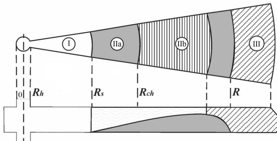
Figure 2 – Scheme of flat radial filtration of mortar in one crack: R_h is hole (well) radius, R_s is radius of sedimentation zone beginning, R_{ch} is radius of channel formation beginning, R is maximum possible radius of mortar extension
