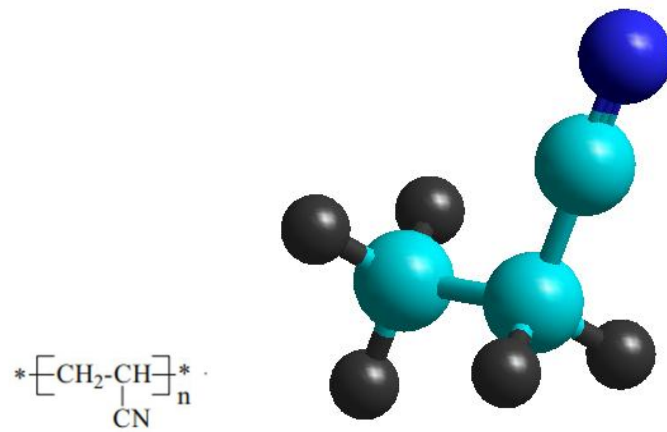
Figure 1 – Optimized model of a monomer of polyacrylonitrile molecule
