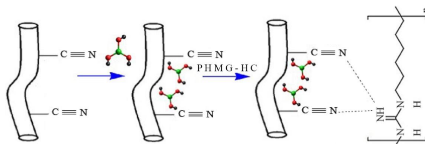
Figure 14 – Modification scheme of ultrafiltration membrane with aluminium oxychloride and polyhexamethylene guanidine hydrochloride (PHMG-HC)
