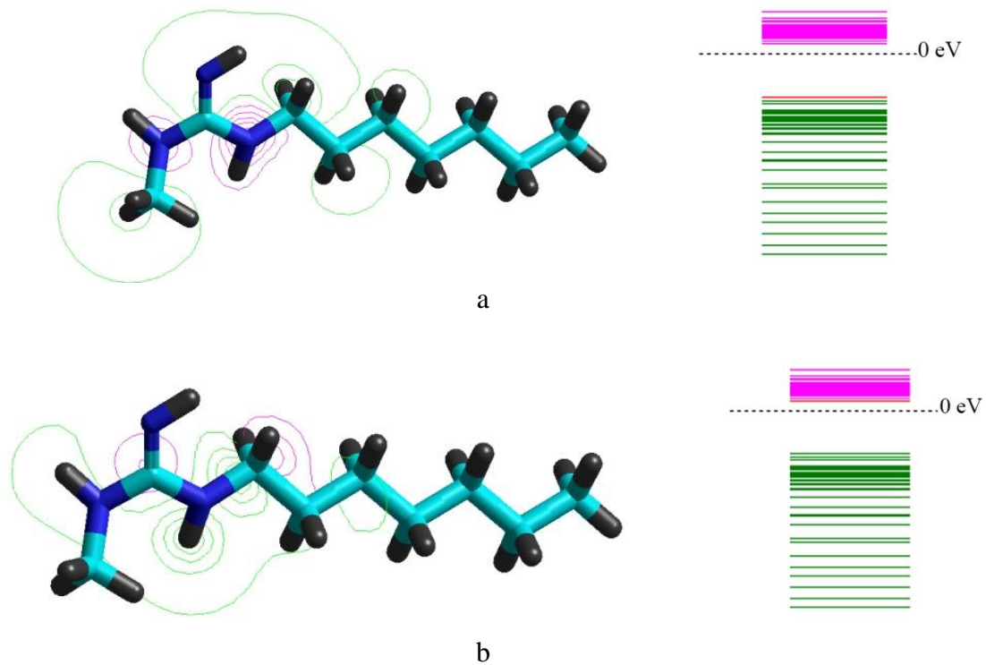
Figure 8 – Distribution of UFMO energy (a) and LVMO energy (b) in the optimized model of monomer of polyhexamethylene guanidine hydrochloride (PHMG-HC)
