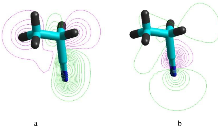
Figure 3 – Distribution of energy UFMO (a) and LVMO (b) in the optimized model of monomer of polyacrylonitrile molecule
