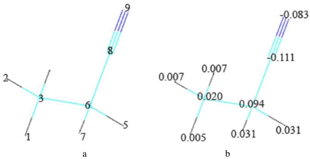
Figure 2 – Numeration of atoms in the model of monomer of polyacrylonitrile molecule (a); charges on atoms (b)
