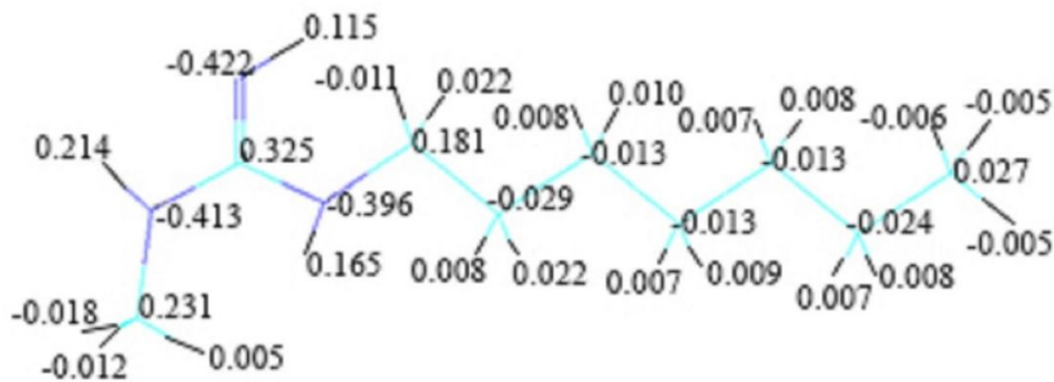
Figure 7 – Charges of atoms in the model of monomer of polyhexamethylene guanidine hydrochloride molecule (PHMG-HC)
