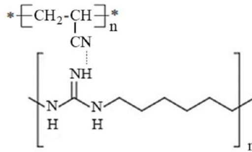
Figure 10 – Interaction scheme of ultrafiltration membrane and polyhexamethylene guanidine hydrochloride (PHMG-HC)
