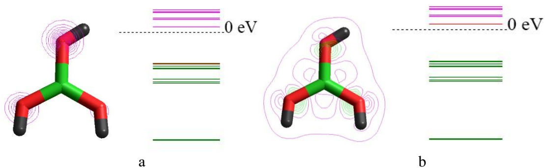
Figure 12 – Distribution of energy UFMO (a) and LVMO (b) in the optimized model of monomer of aluminium oxychloride molecule
