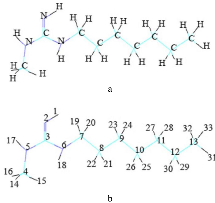
Figure 6 – The symbols of atoms (a) and numeration of atoms (b) in the model of monomer of PHMG-HC molecule.
