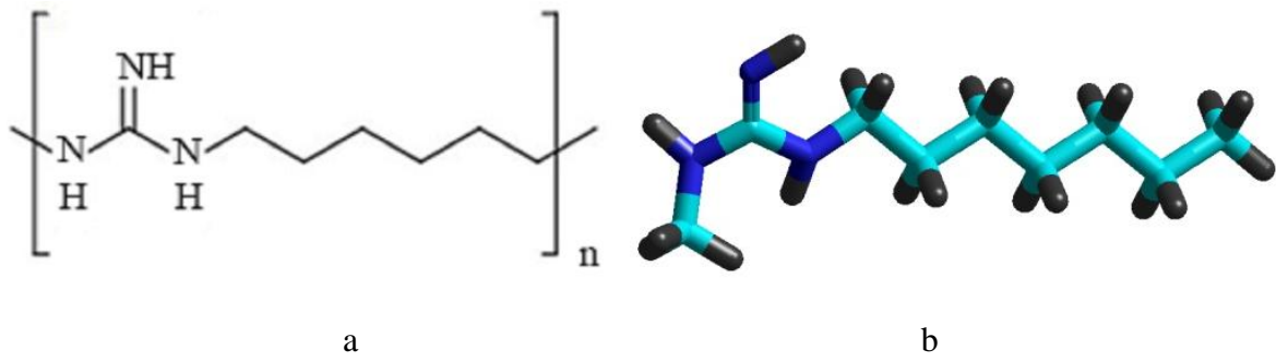
Figure 5 – The monomer PHMG-HC (a) and the optimized model of monomer of polyhexamethylene guanidine hydrochloride molecule (b)
