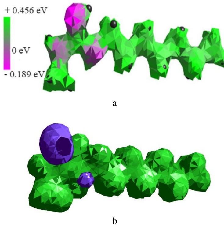
Figure 9 – Distribution of electrostatic potential in the optimized model of monomer of polyhexamethylene guanidine hydrochloride molecule (PHMG-HC) (a) and isosurface (b)
