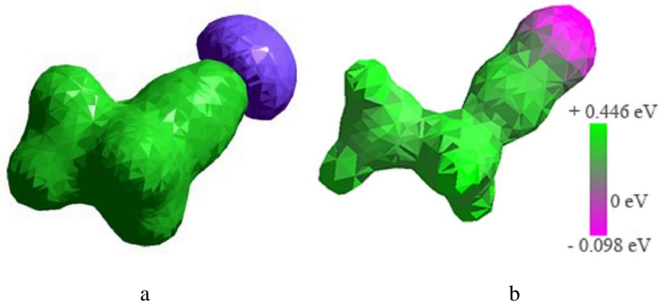
Figure 4 – Distribution of electrostatic potential in the optimized model of monomer of polyacrylonitrile molecule (a) and isosurface (b)
