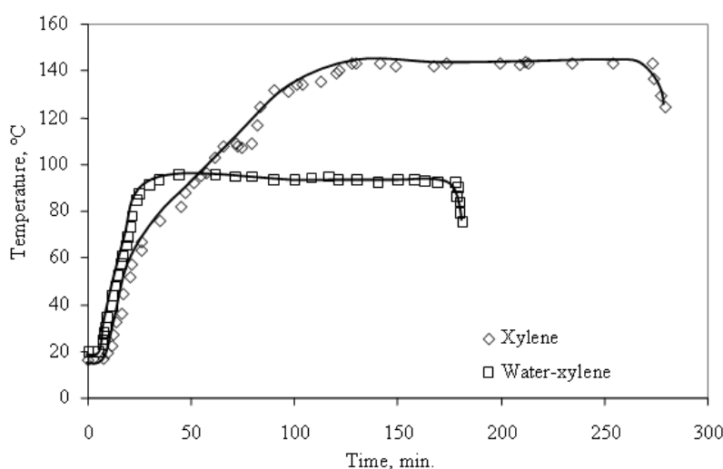
Figure 1 – Thermal regime of natural rubber epoxidation
