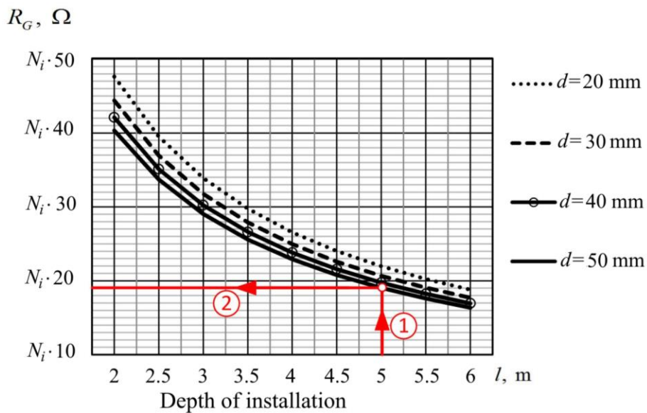
Figure 2 – Universal graphical dependencies R_G = f(l) , for different values of the electrode's diameter and arbitrary value of soil's resistivity and its corresponding number N_i
