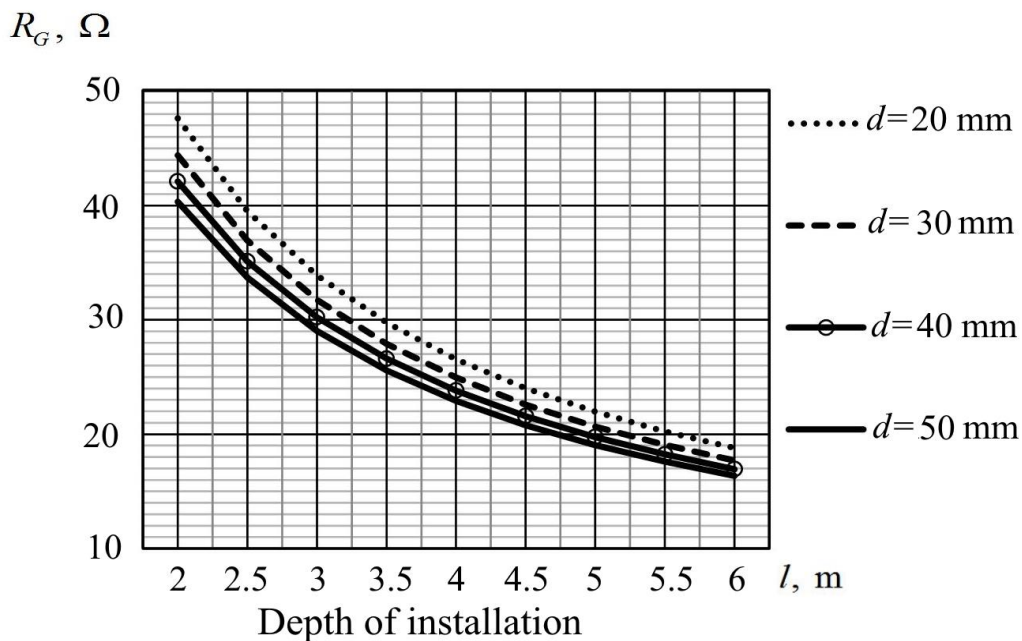
Figure 1 – Graphical dependencies R_G = f(l) , for different values of the electrode's diameter and a fixed soil resistivity of \rho_S = 100 \text{ } \Omega \cdot \text{m}
