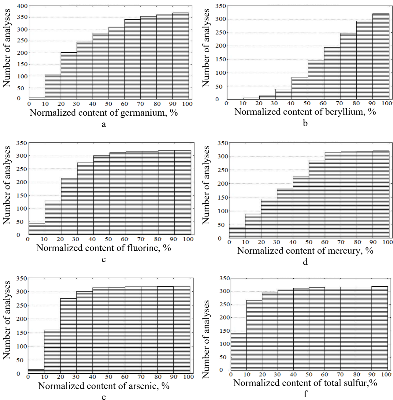
a – Ge, b – Be, c – F, d – Hg, e – As, f – total sulfur Figure 1 – Cumulative histograms of normalized content values
