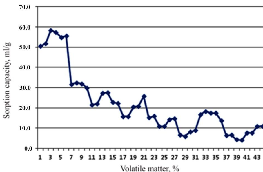
Figure 1 – Graph of the sorption capacity of coal depending on the degree of metamorphism.
