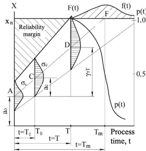
Figure 5 – Schematic diagram of progressive failure formation
