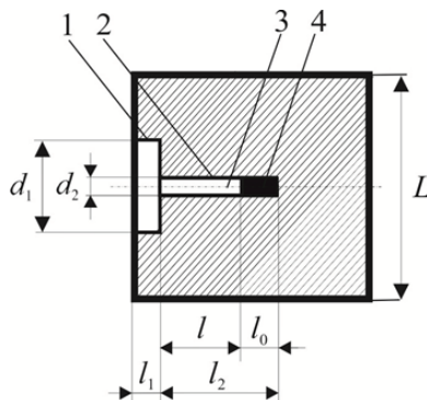
1 – cavity simulating part of the mine working; 2 – charging cavity simulating a borehole; 3 – stemming; 4 – explosive charge; d_1 , d_2 – cavity diameters, m; l_1 , l_2 – cavity lengths, m; l_0 – length of the explosive charge, m; l – stemming length, m
