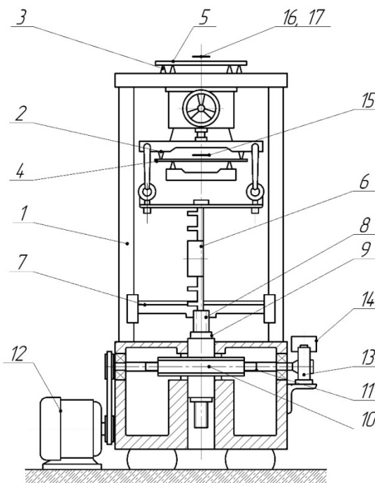
1 – frame; 2, 3 – rismatic supports; 4, 5 – elastic sensing elements; 6 – rubber sample of a grate-card element; 7 – movable traverse; 8 – lead screw; 9 – nut; 10 – worm gear; 11 – worm; 12 – electric motor; 13 – brake; 14 – electromagnetic drive; 15 – 16 – 17 groups of strain gauges
