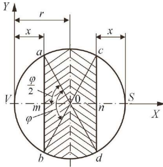
Figure 3 – Diagram showing the formation of the bearing area during the development of two symmetrical cracks in a cylindrical specimen
