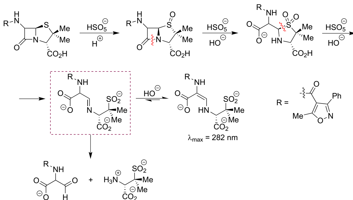
Figure 2. The scheme of coupled reactions of peroxyacid oxidation and perhydrolysis of sulfon Oxa with the formation of a substituted derivative of N-acryl- \beta -penicillamine sulfate
