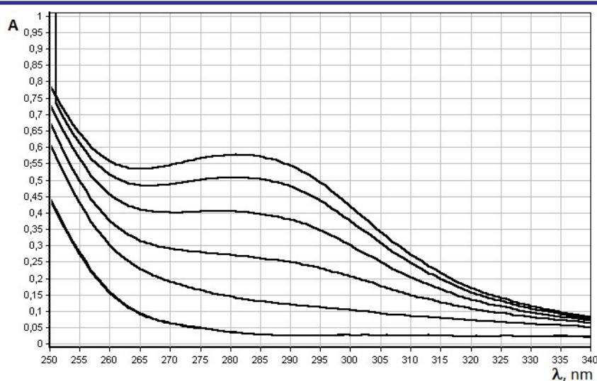
Figure 1. Electronic light absorption spectra of the reaction product of alkaline hydrolysis and Oxa perhydrolysis of the sodium salt over time. c(\text{NaOH}) = 6.1 \times 10^{-3} \text{ mol L}^{-1} ; c(\text{KHSO}_5) = 1.2 \times 10^{-3} \text{ mol L}^{-1} ; c(\text{Oxa}) = 30 \text{ mg mL}^{-1}
