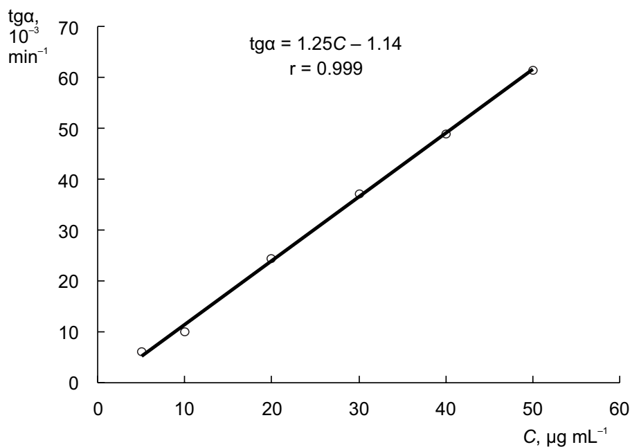
Figure 3. The calibration graph for the quantitative determination of Oxa, c(\text{KHSO}_5) = 2 \times 10^{-3} \text{ mol L}^{-1} ; c(\text{NaOH}) = 6.1 \times 10^{-3} \text{ mol L}^{-1}
