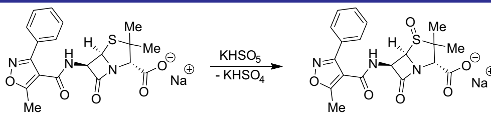
Figure 4. The scheme of S-oxidation of Oxa by Potassium hydrogen peroxomonosulfate
