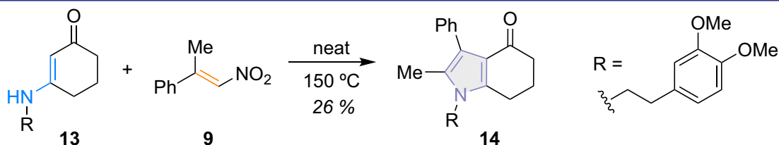
Scheme 4. The synthesis of pyrrole from enaminone based on dimedone
