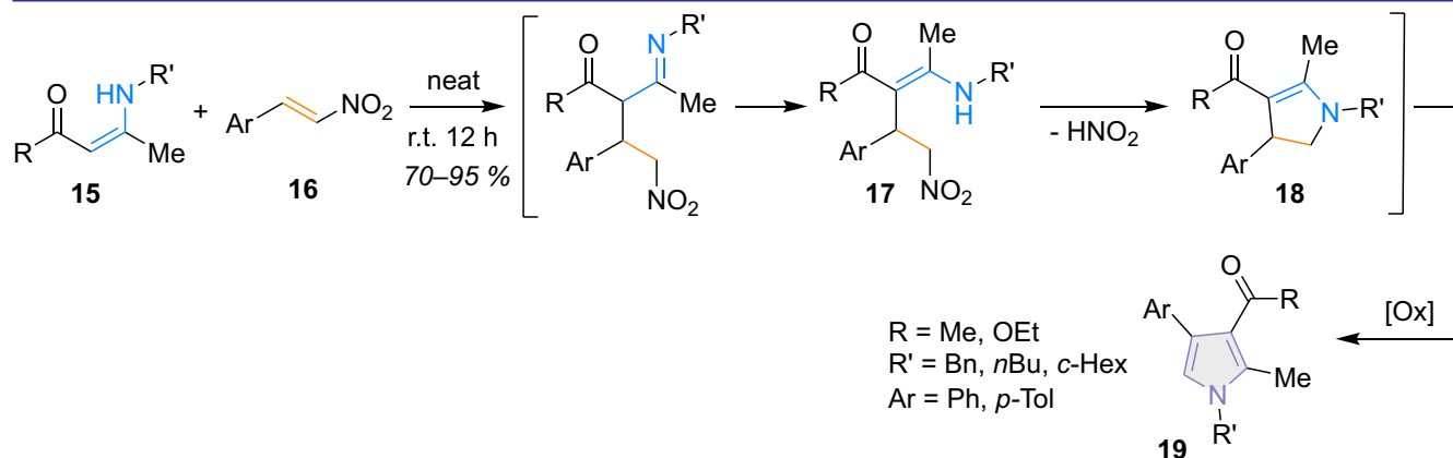
Scheme 5. The reaction mechanism of the pyrrole formation in the reaction between enaminones and nitrostyrenes
