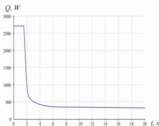
Fig. 6 – Time dependence of thermal power of pyrotechnic heat source.
