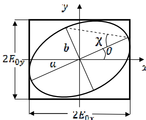
Fig. 5. Polarization ellipse
