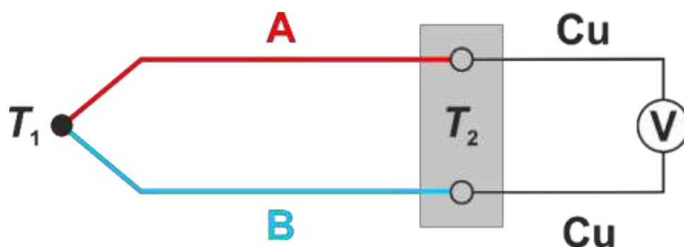
Fig. 2. Basic circuit of temperature measurement with thermocouples
