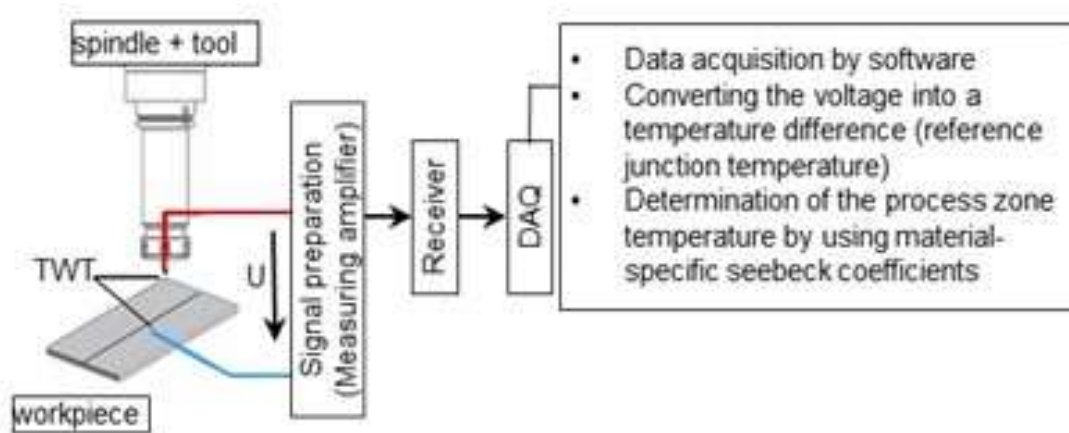
Fig. 3. Basic principle of the Tool-Workpiece- Thermocouple (TWT) Method [11]
