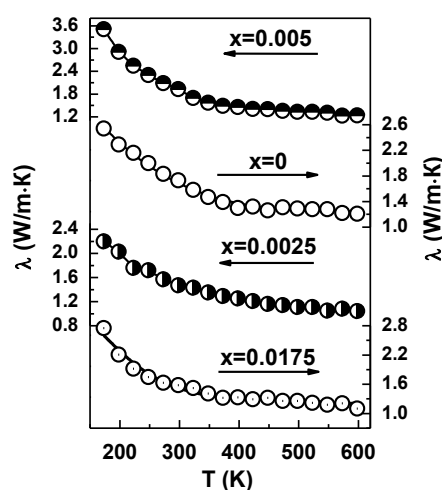
Fig. 2. Temperature dependences of total thermal conductivity \lambda of \text{PbSe}_{1-x}\text{Te}_x solid solution
