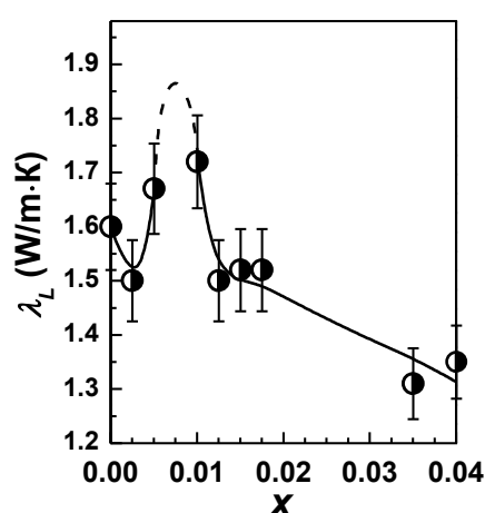
Fig. 1. Dependence of lattice thermal conductivity \lambda_L of \text{PbSe}_{1-x}\text{Te}_x solid solution on the composition x at a temperature of 325 K
