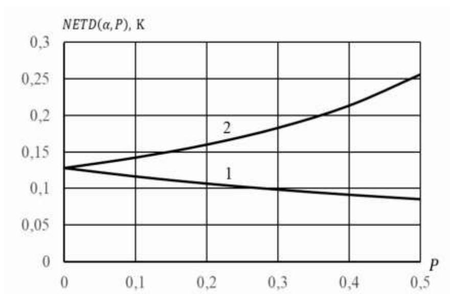
Fig. 2. Dependence of the temperature resolution of the polarization thermal imager on the degree of polarization P of test object radiation for the angular orientation \alpha of the polarizer relative to the optical axis of the phase plate which is equal to: 1 – 0^\circ ; 2 – 90^\circ
