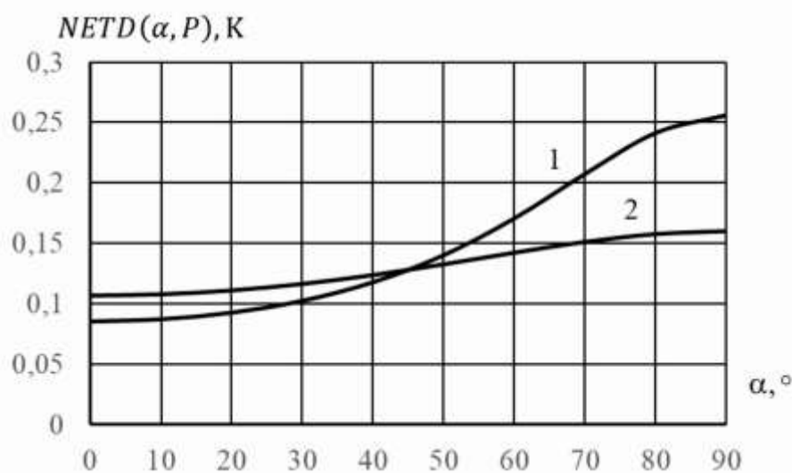
Fig. 3. Dependence of temperature resolution of the polarization thermal imager on the angular orientation \alpha of the polarizer relative to optical axis of the phase plate for the degree of polarization: 1 – P = 0.5 ; 2 – P = 0.2 .
