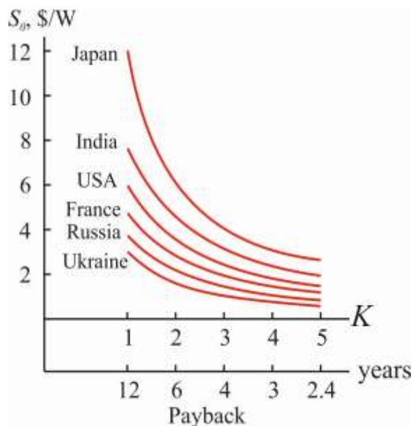
Fig. 2. Reasonable unit cost of TEG depending on the payback period.
