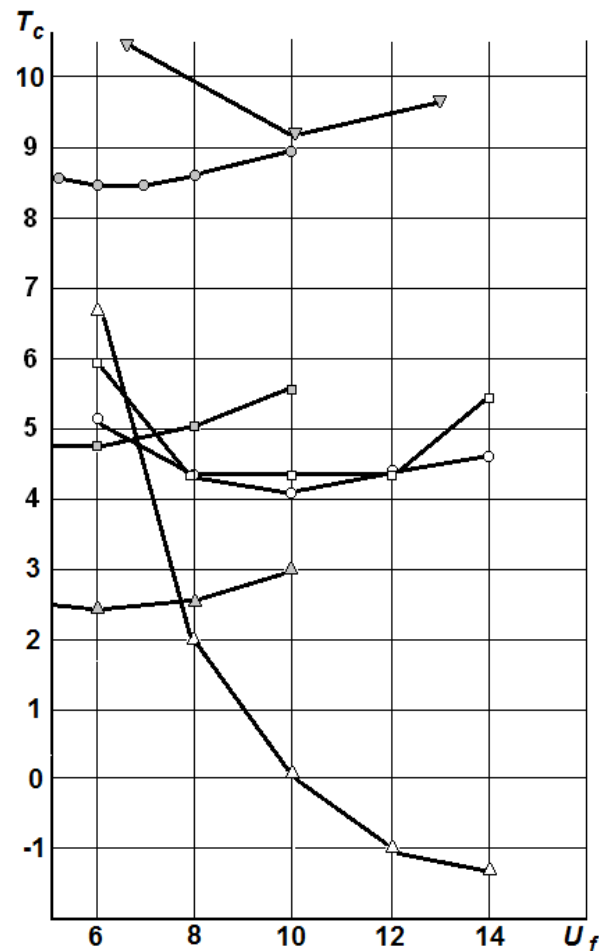
Fig.4. Dependence of the container (chamber) temperature T_c on the supply voltage of fan U_f Installed on the hot side of the module at different values of its supply voltage, namely: ○ - U_m = 6V ; □ - U_m = 8V ; △ - U_m = 10V ; the rest of the graphs and symbols relate to the comparison of results with the data of other studies, and are explained in the text.
