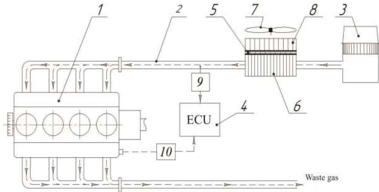
Fig. 3. Block-diagram of the proposed thermoelectric system:
