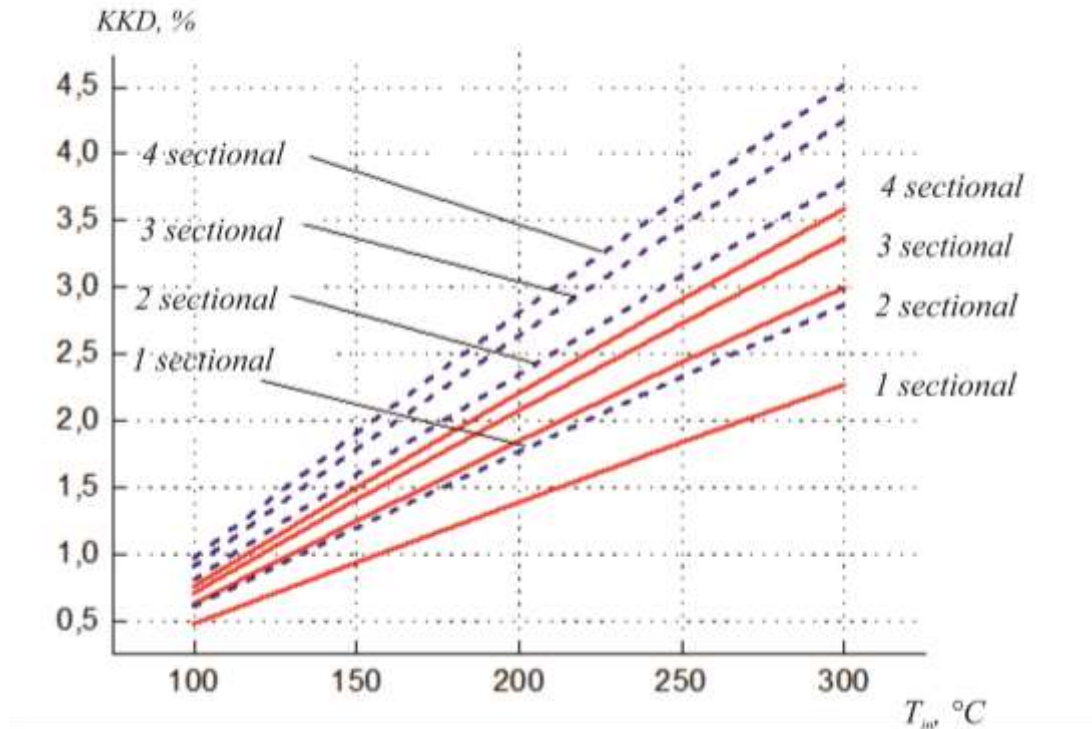
Fig. 5. The efficiency of sectional TEC with regard to heat exchange (solid lines) and without heat exchange (dashed lines). The height of thermoelement legs is 1 cm.
