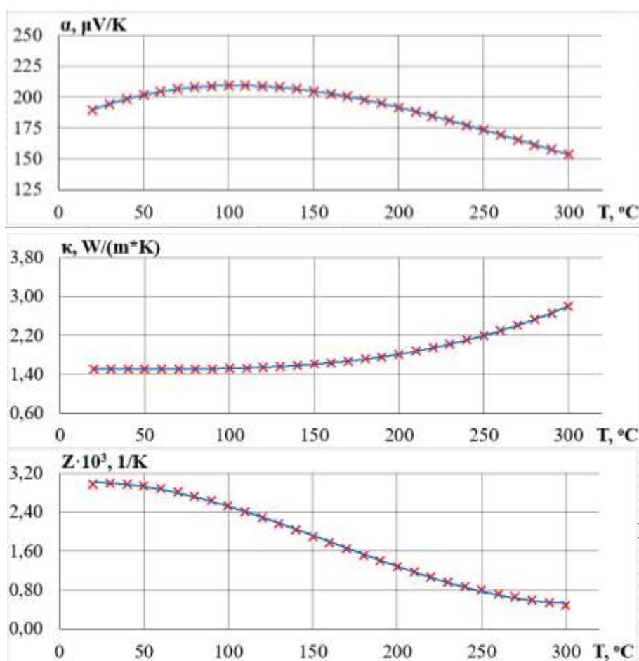
Fig. 3. Temperature dependences of the thermoelectric properties of Bi-Te based material (the lines indicate the dependences constructed using polynomials (5)-(8), the marks "x" are the results obtained by a computer experiment using the proposed measurement technique).
