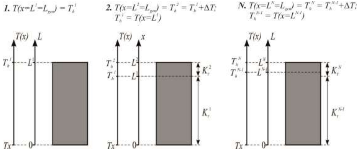
Fig. 2. Procedure for determining the thermal conductivity of the legs material with a rise in temperature difference
