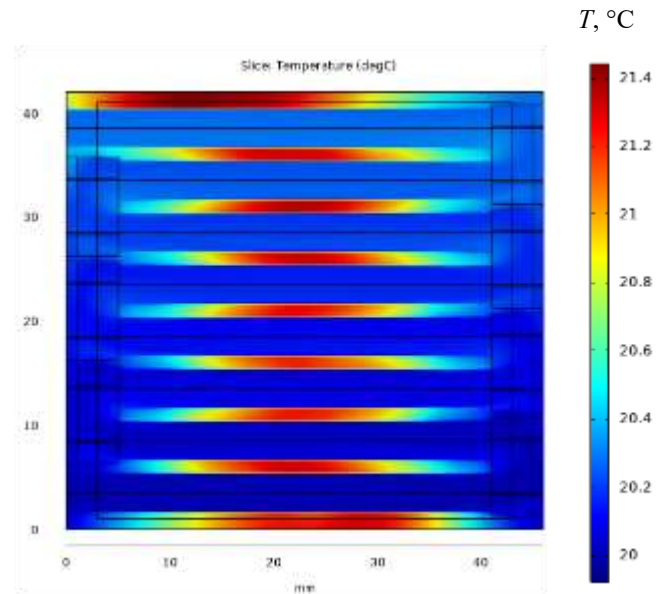
Fig. 8. Example of distribution of heat carrier temperature in the cold heat exchanger of thermoelectric generator
