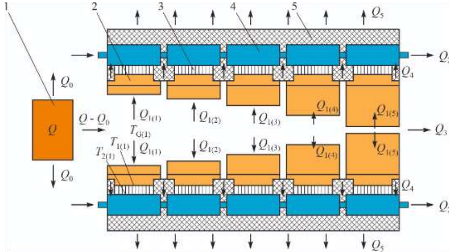
Fig. 1. Physical model of a thermoelectric generator for heat and electricity source for armoured vehicles.: 1 – heat source; 2 – hot heat exchanger (radiator); 3 – thermopile; 4 – cold heat exchanger; 5 – thermal insulation
