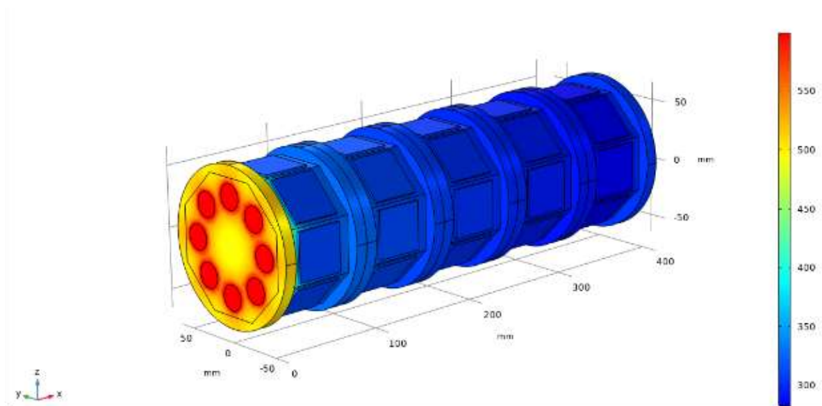
Fig. 4. Example of temperature distribution in the hot heat exchanger of the generator
