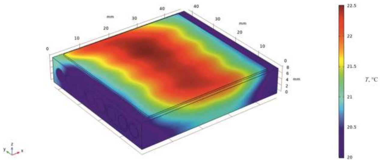
Fig. 6. Example of temperature distribution in the hot heat exchanger of the generator
