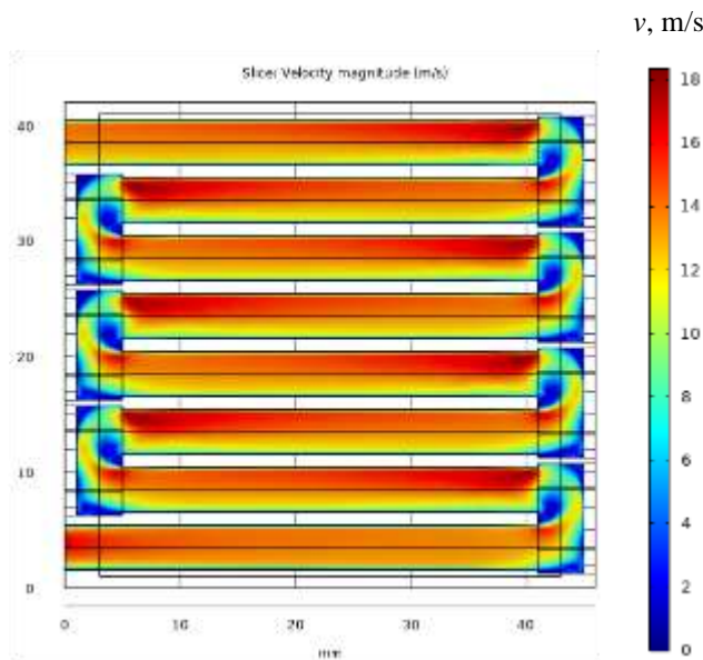
Fig. 7. Example of distribution of heat carrier velocity in the cold heat exchanger of thermoelectric generator
