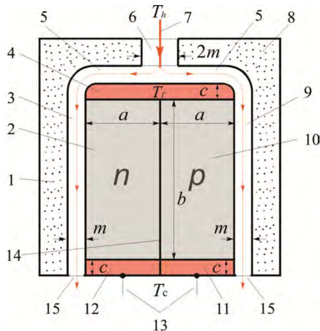
Fig. 1. Physical model of a permeable thermoelement:
