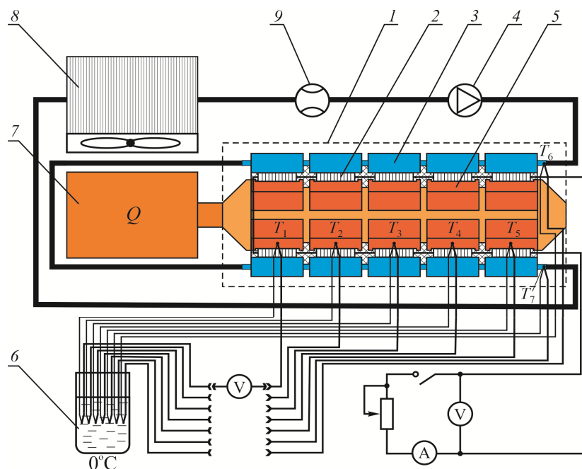
Fig. 3. Layout of the bench for experimental studies of characteristics of the developed model sample of thermoelectric generator: 1 –thermoelectric generator; 2 – thermoelectric modules; 3 – cold heat exchangers; 4 – circulation pump; 5 – hot heat exchangers; 6 – Dewar vessel; 7 – heat source on diesel fuel; 8 – radiator
