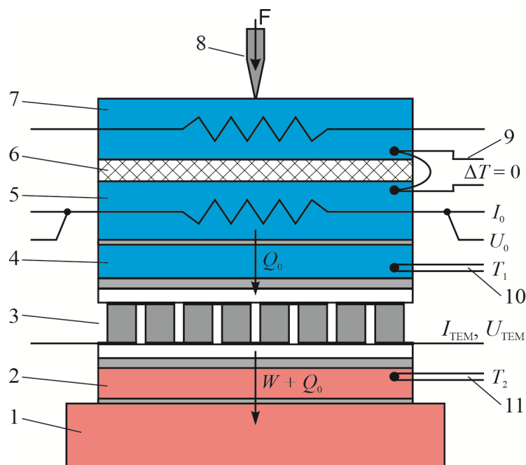
Fig. 1. Absolute method of measuring the parameters of thermoelectric cooling modules:
