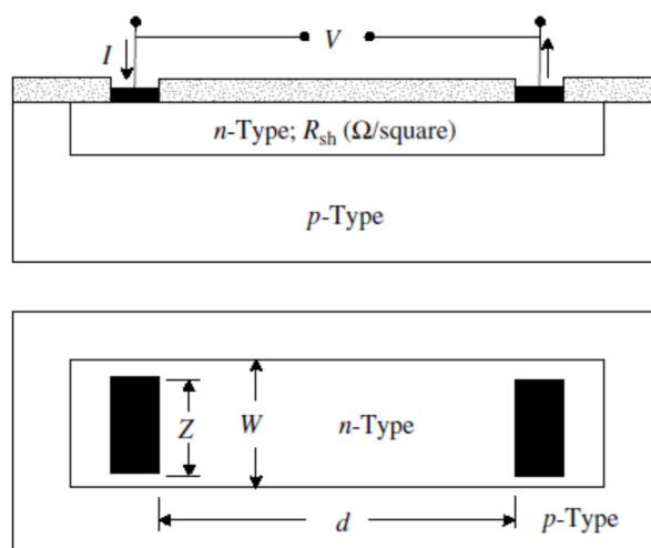
Fig. 2. Surface (horizontal) structure for implementing the two-terminal method of measuring contact resistance in section and plan view [10].
