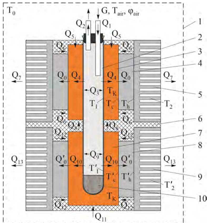
Fig. 1 – Physical model of a cooling unit for a thermoelectric device for collecting condensate from the air exhaled by a person: 1 – thermostat (device body); 2 – test tube for collecting condensate; 3 – working chamber; 4, 8 – thermoelectric modules; 5, 9 – air heat exchangers; 6 – thermal insulation; 7 – additional cooling chamber; 10 – collected moisture
