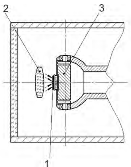
Fig. 1. The simplest model of IR device with TEC [9]. 1 – IR detector with TEC, 2 – lens, 3 – heat-receiving base
