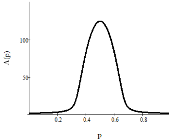
Fig. 1. Concentration dependence of the product of effective conductivities in a three-dimensional random-inhomogeneous medium. For example, \sigma_1 = 1 , \sigma_2 = 10^{-2} is selected (in conventional units)
