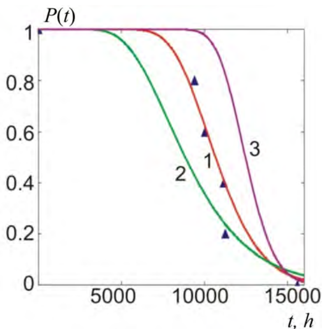
Fig. 1. Dependences of the probability of saving 80% of the output power of thermoelectric energy converters on the time of operation: 1 – the most probable in accordance with the diffusion-nonmonotonic of the distribution of failure times, 2, 3 – limit at a confidence probability of 0.95, triangles – the result of predicting the time of saving 80 % of the output power according to the probabilistic theory of degradation
