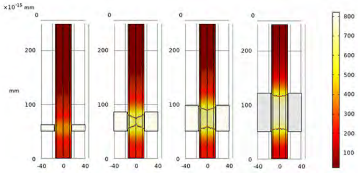
Fig. 2. Computer model of change in the shape of crystallization front
